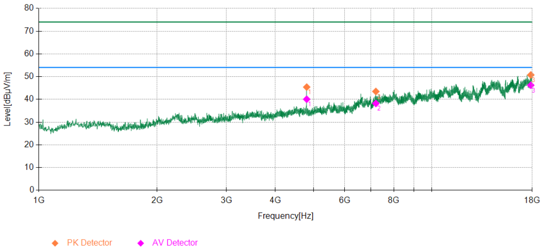
Low Channel - 1-18 GHz - Horizontal
