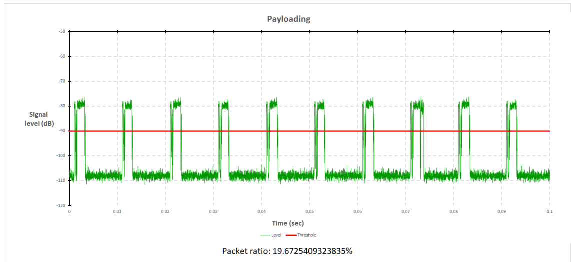
Plot of Slave Traffic at 5570 MHz
