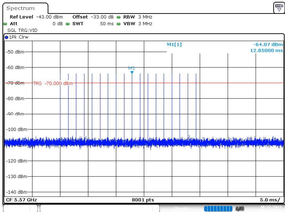
Radar Type 0 Calibration Plot (5570 MHz)
