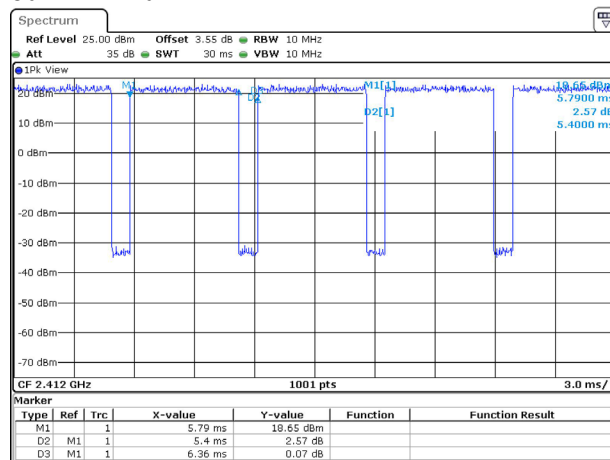
802.11ax-20 MHz
