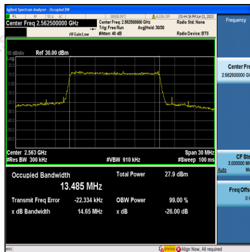
Band7-15MHz-16QAM-21375-75RB#0-13.485
