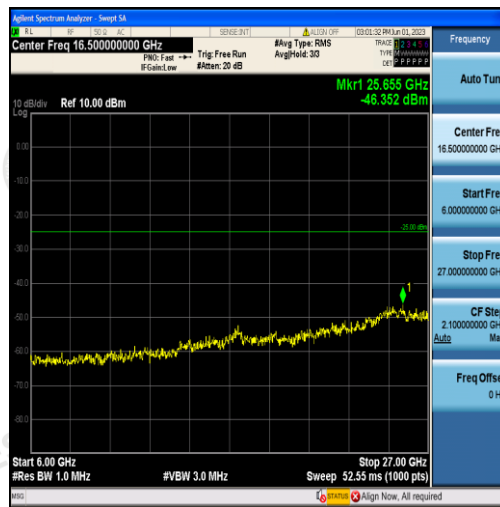
Band7-5MHz-16QAM-21100-25RB#0-Range3:6000~27000MHz
