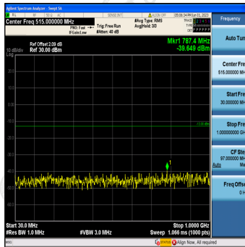
Band66-5MHz-QPSK-131997-25RB#0-Range1:30~1000MHz
