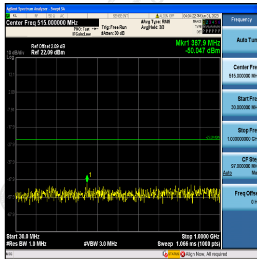
Band7-20MHz-16QAM-21100-100RB#0-Range1:30~1000MHz
