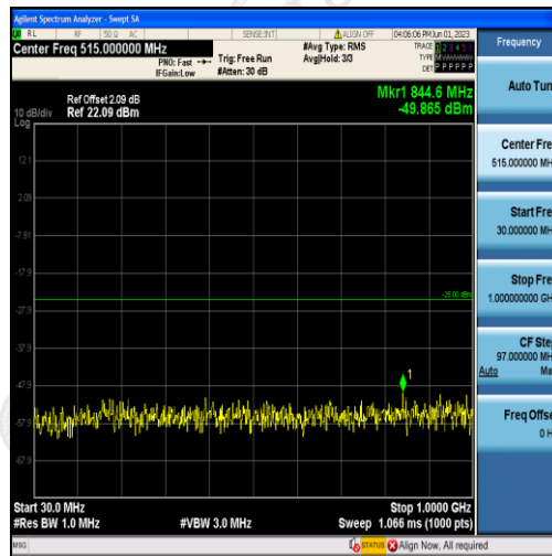
Band7-20MHz-16QAM-21350-100RB#0-Range1:30~1000MHz
