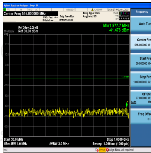
Band66-3MHz-16QAM-131987-15RB#0-Range1:30~1000MHz
