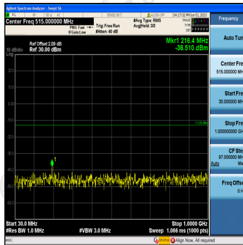
Band66-1.4MHz-QPSK-131979-6RB#0-Range1:30~1000MHz
