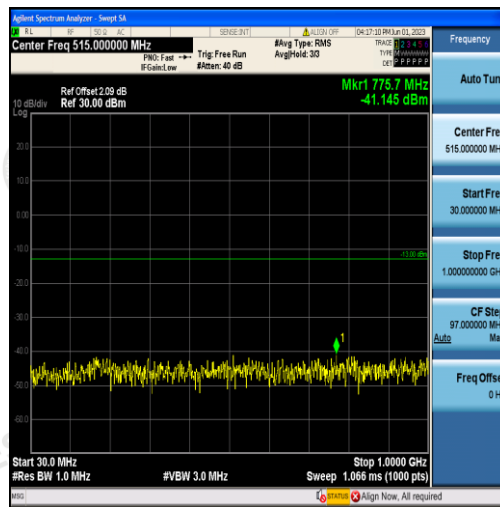
Band66-1.4MHz-16QAM-131979-6RB#0-Range1:30~1000MHz
