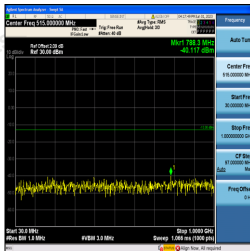
Band66-1.4MHz-16QAM-132665-6RB#0-Range1:30~1000MHz
