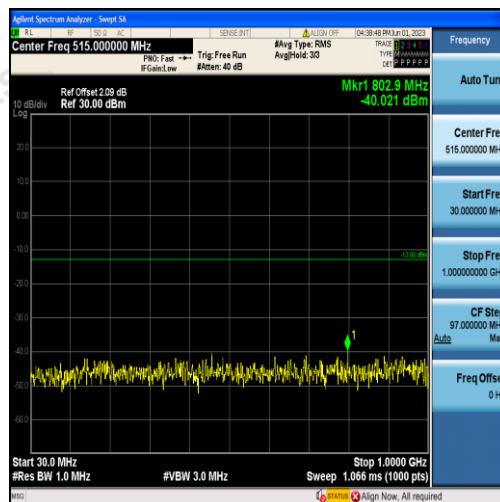
Band66-3MHz-QPSK-132322-15RB#0-Range1:30~1000MHz
