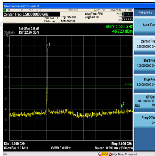
Band7-15MHz-QPSK-21100-75RB#0-Range2:1000~6000MHz
