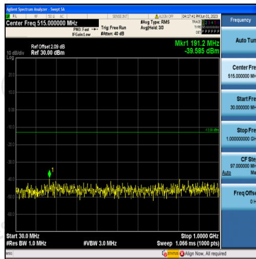
Band66-1.4MHz-QPSK-132665-6RB#0-Range1:30~1000MHz
