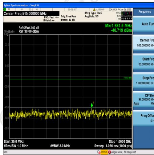
Band66-3MHz-QPSK-131987-15RB#0-Range1:30~1000MHz
