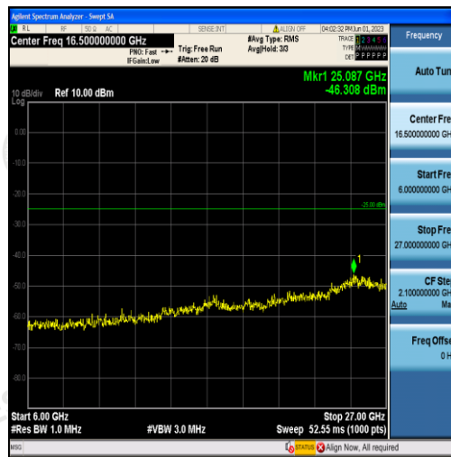
Band7-20MHz-16QAM-20850-100RB#0-Range3:6000~27000MHz
