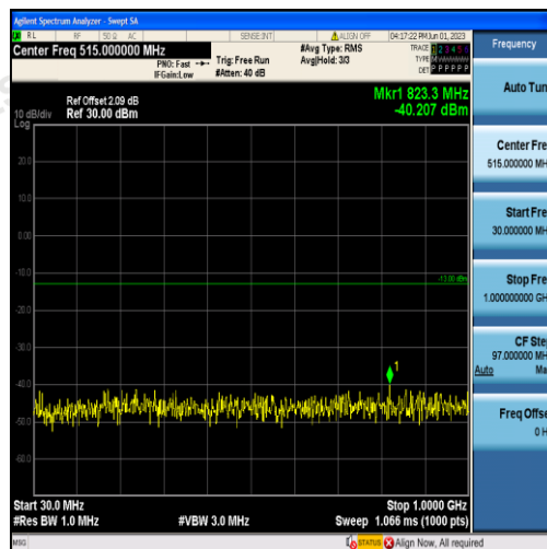
Band66-1.4MHz-QPSK-132322-6RB#0-Range1:30~1000MHz
