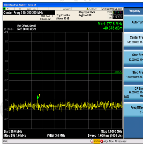
Band66-3MHz-16QAM-132322-15RB#0-Range1:30~1000MHz
