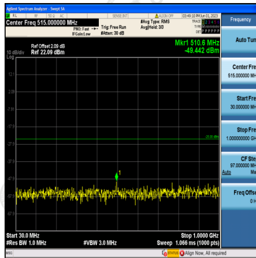
Band7-15MHz-QPSK-21100-75RB#0-Range1:30~1000MHz
