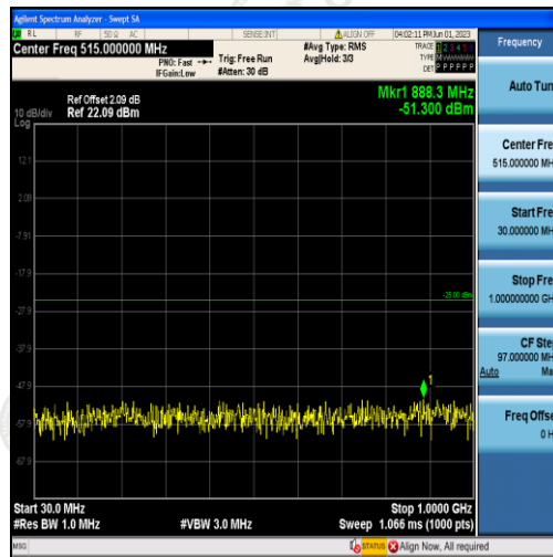
Band7-20MHz-16QAM-20850-100RB#0-Range1:30~1000MHz
