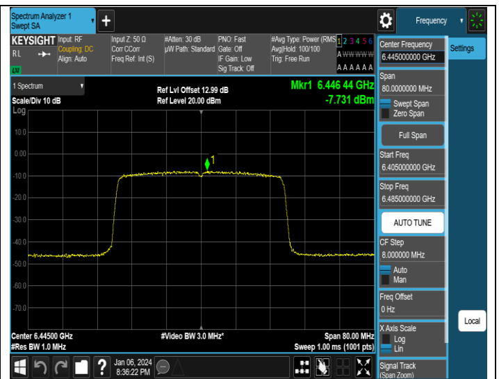
11AX40SISO-Ant4-6445-PASS
