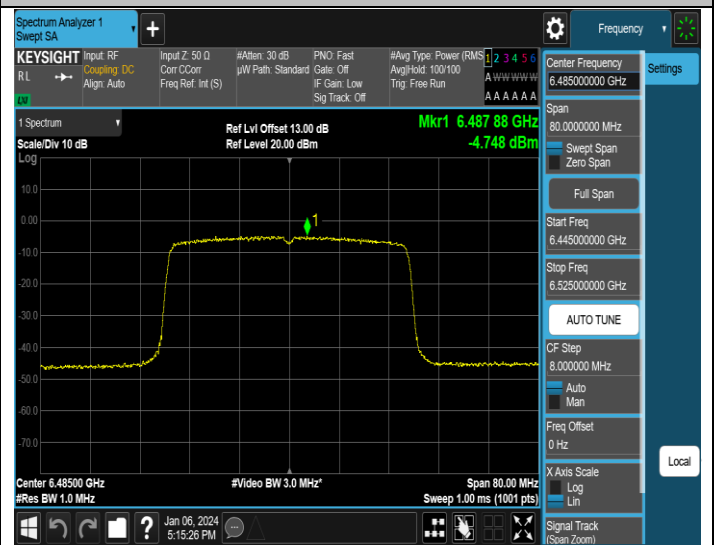
11AX40SISO-Ant2-6485-PASS
