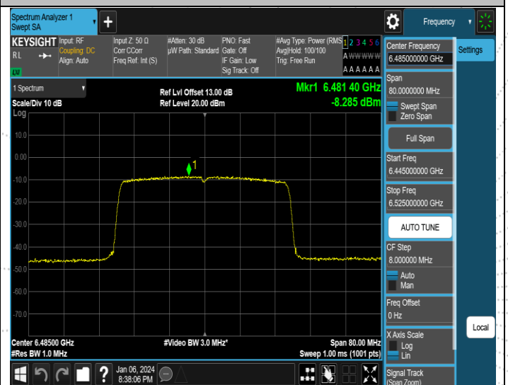
11AX40SISO-Ant4-6485-PASS
