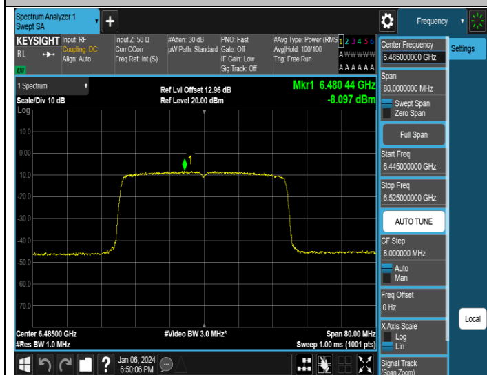
11AX40SISO-Ant3-6485-PASS
