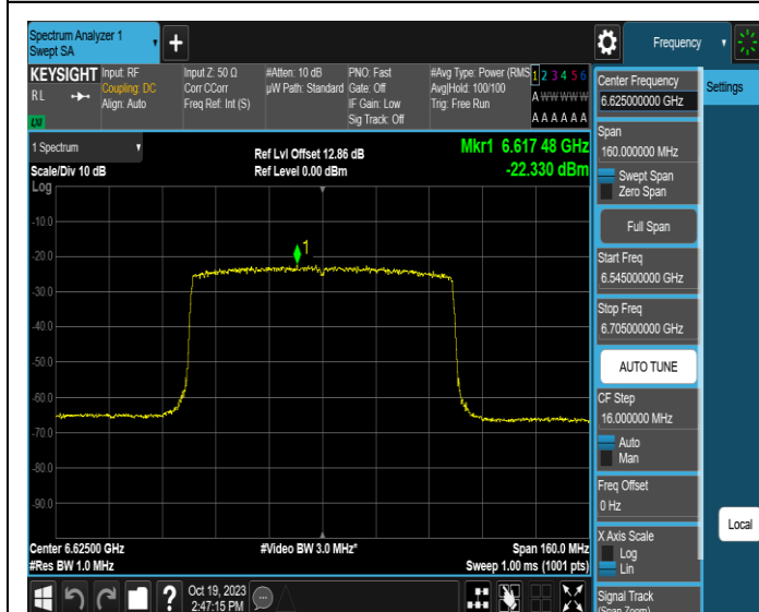
11AX80MIMO-Ant3-6625-PASS
