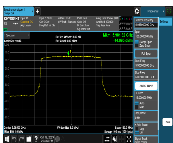
11AX80MIMO-Ant2-5985-PASS
