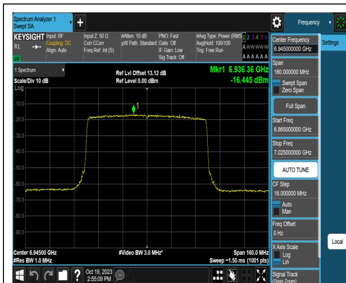
11AX80MIMO-Ant1-6945-PASS
