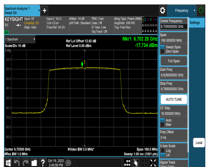
11AX80MIMO-Ant4-6705-PASS
