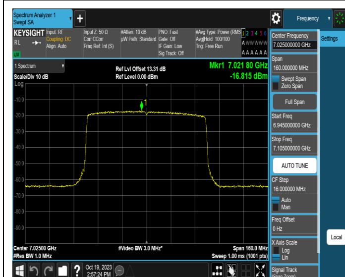
11AX80MIMO-Ant1-7025-PASS
