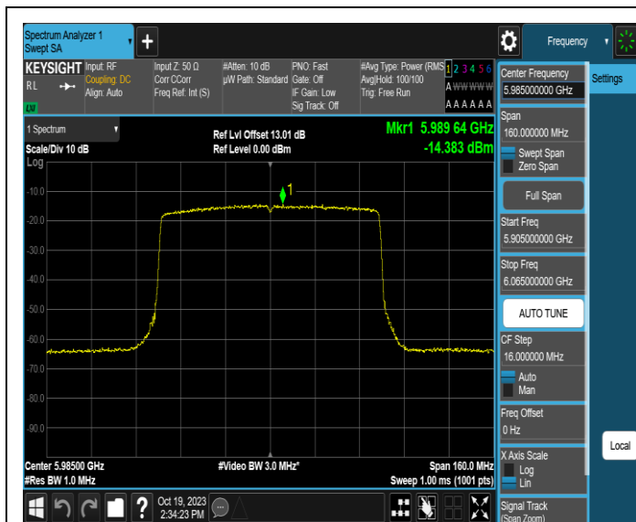
11AX80MIMO-Ant1-5985-PASS
