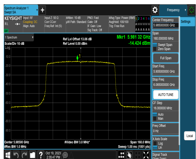
11AX80MIMO-Ant4-5985-PASS
