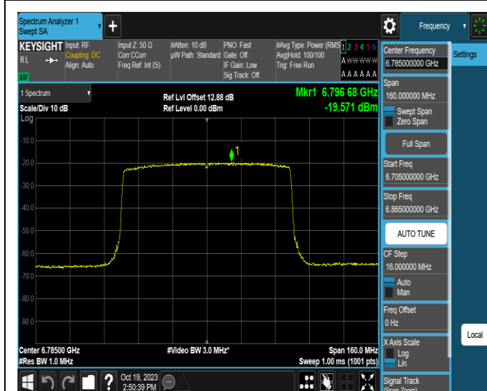
11AX80MIMO-Ant1-6785-PASS
