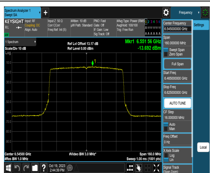
11AX80MIMO-Ant2-6545-PASS
