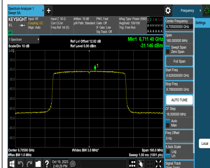
11AX80MIMO-Ant3-6705-PASS
