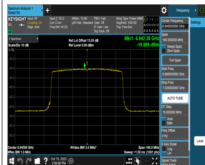
11AX80MIMO-Ant3-6945-PASS
