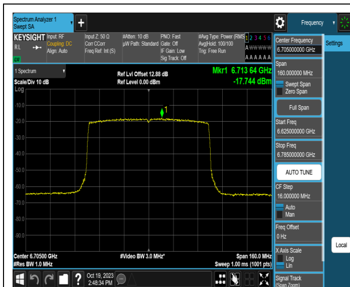
11AX80MIMO-Ant1-6705-PASS
