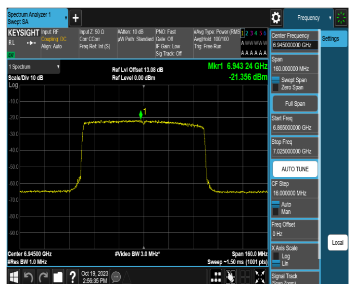
11AX80MIMO-Ant4-6945-PASS
