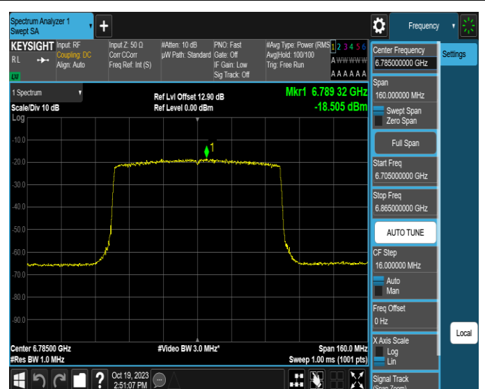
11AX80MIMO-Ant2-6785-PASS
