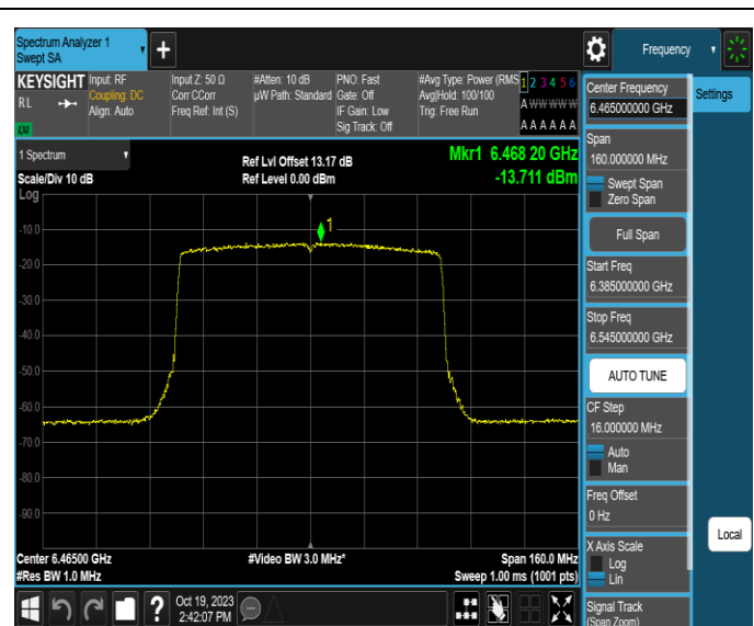
11AX80MIMO-Ant2-6465-PASS
