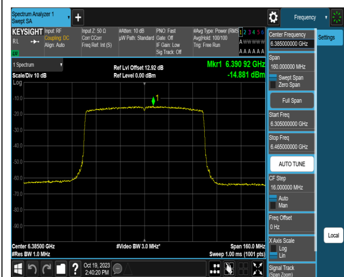
11AX80MIMO-Ant3-6385-PASS
