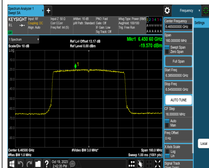
11AX80MIMO-Ant3-6465-PASS
