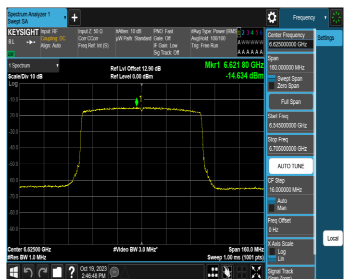
11AX80MIMO-Ant2-6625-PASS
