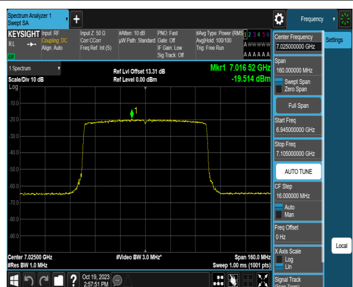
11AX80MIMO-Ant2-7025-PASS
