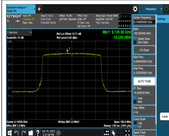
11AX80MIMO-Ant1-6145-PASS
