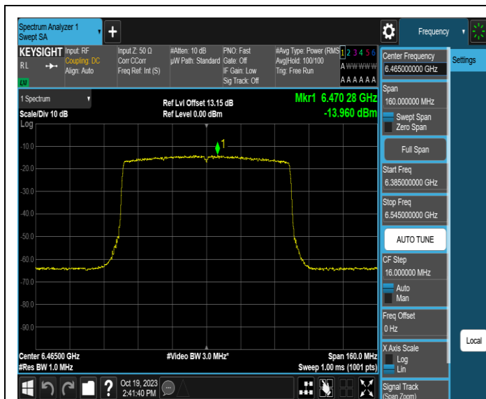
11AX80MIMO-Ant1-6465-PASS
