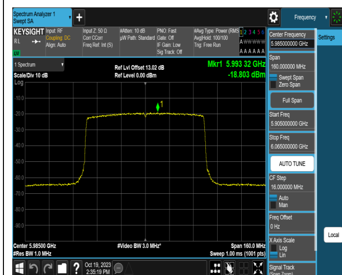
11AX80MIMO-Ant3-5985-PASS
