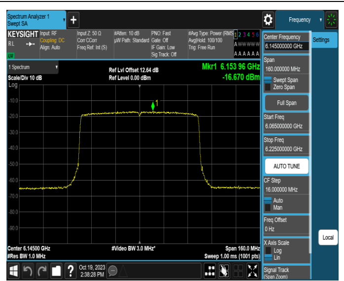
11AX80MIMO-Ant4-6145-PASS
