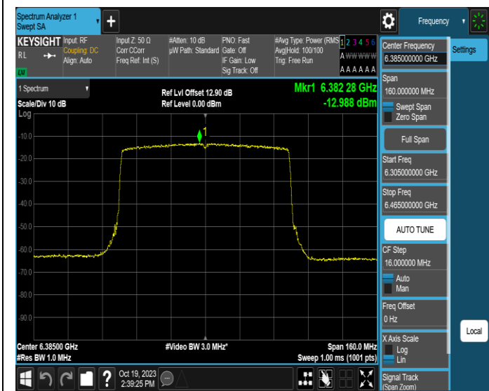
11AX80MIMO-Ant1-6385-PASS
