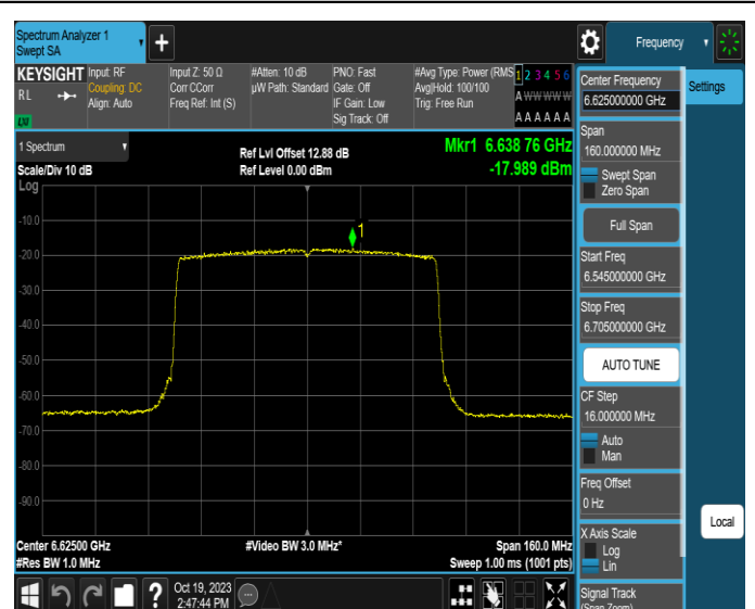
11AX80MIMO-Ant4-6625-PASS
