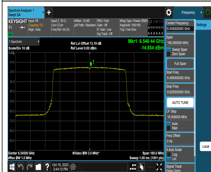
11AX80MIMO-Ant1-6545-PASS
