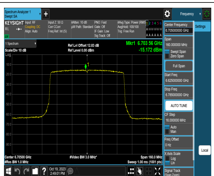
11AX80MIMO-Ant2-6705-PASS
