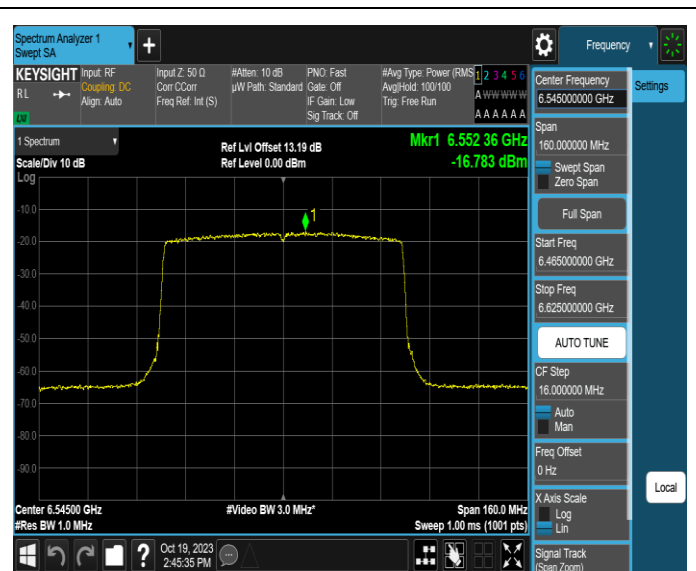
11AX80MIMO-Ant4-6545-PASS
