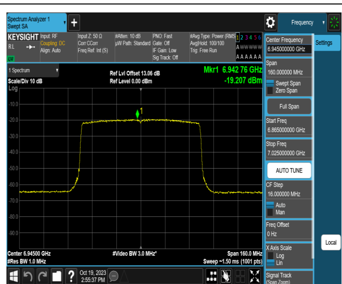
11AX80MIMO-Ant2-6945-PASS
