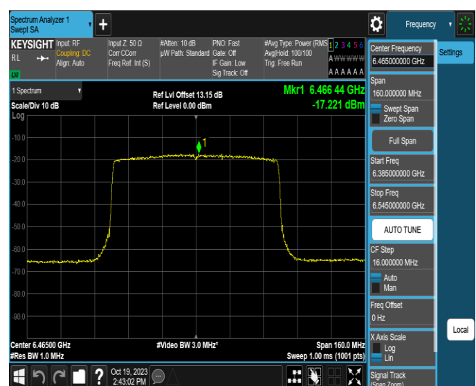
11AX80MIMO-Ant4-6465-PASS
