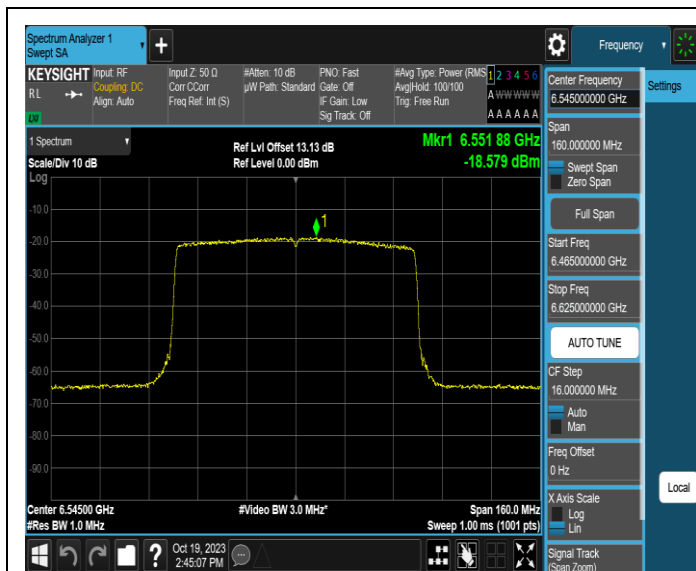
11AX80MIMO-Ant3-6545-PASS
