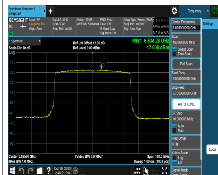
11AX80MIMO-Ant1-6625-PASS
