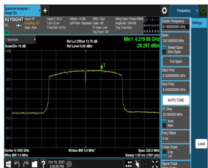
11AX160MIMO-Ant2-6185-PASS
