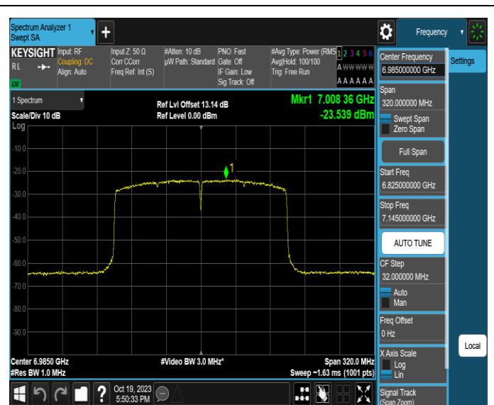
11AX160MIMO-Ant2-6985-PASS
