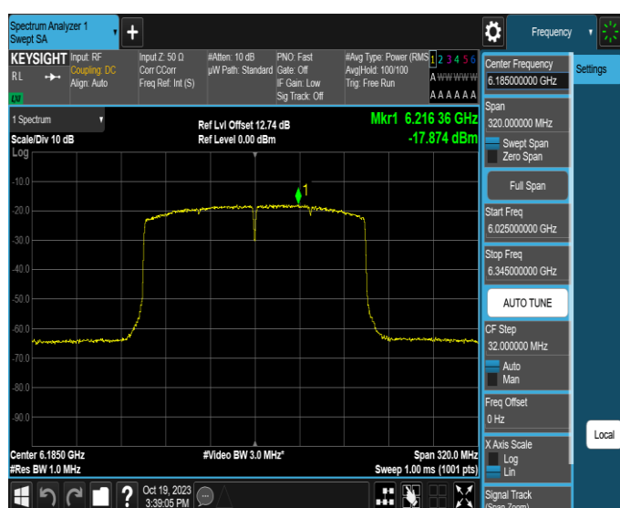
11AX160MIMO-Ant1-6185-PASS
