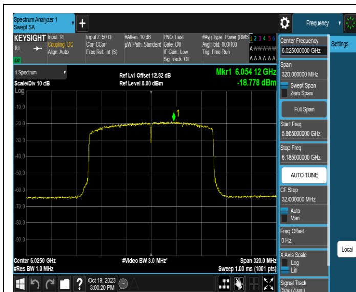
11AX160MIMO-Ant1-6025-PASS
