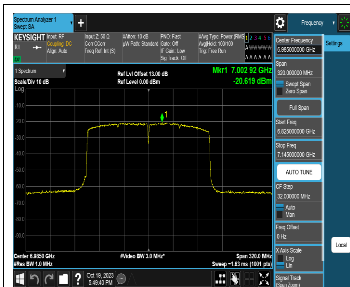
11AX160MIMO-Ant1-6985-PASS
