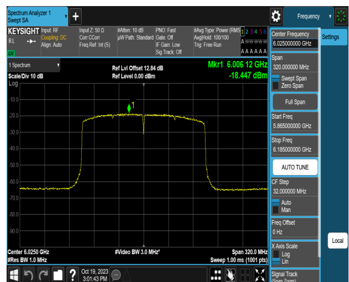
11AX160MIMO-Ant4-6025-PASS
