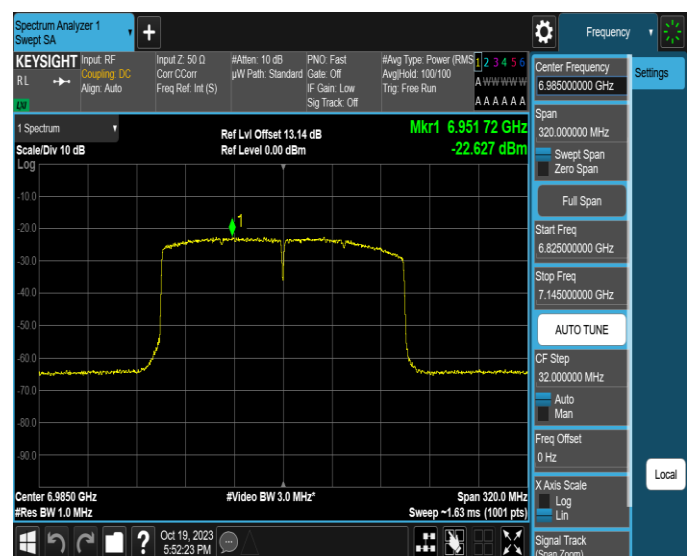
11AX160MIMO-Ant4-6985-PASS
