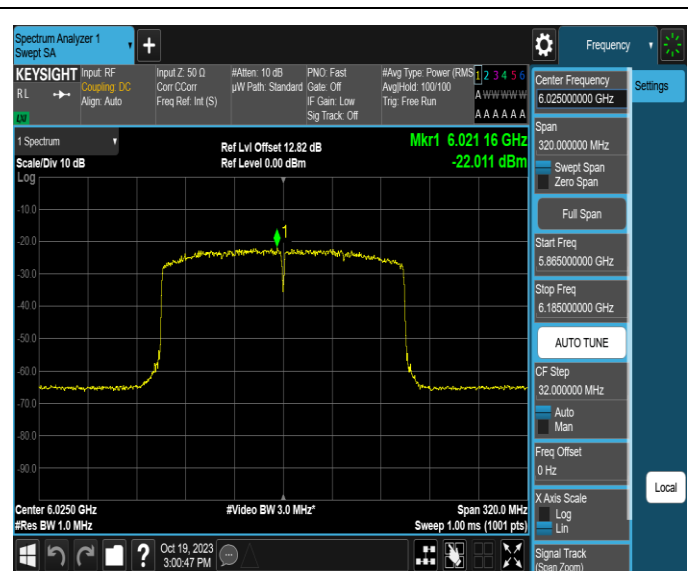
11AX160MIMO-Ant2-6025-PASS
