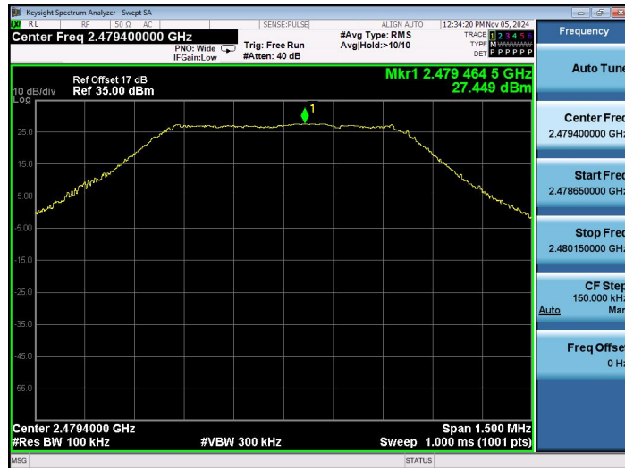
2.4G-Ant2-2479.4-0~Reference-PASS
