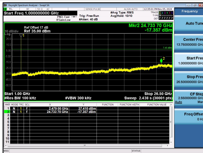
2.4G-Ant2-2479.4-1000~26500-PASS
