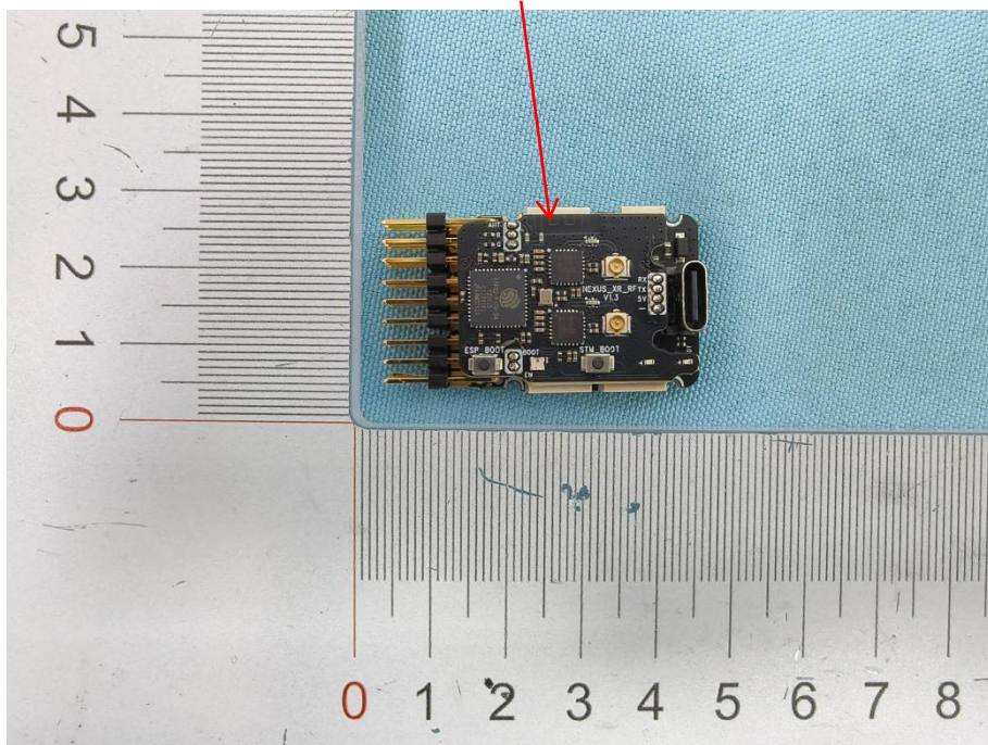
WIFI+BDR+EDR ANT
