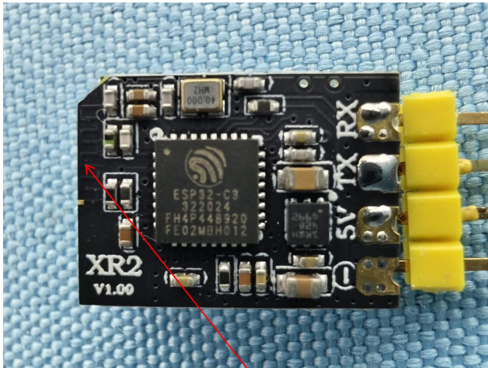
WiFi-ANT
