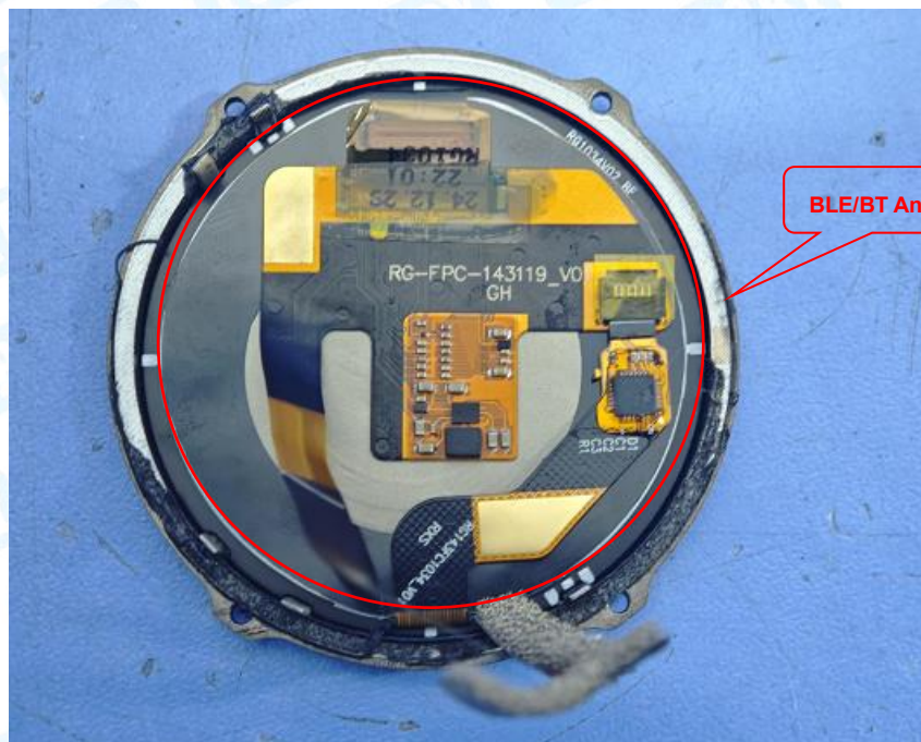
Photo 15 Internal of EUT
