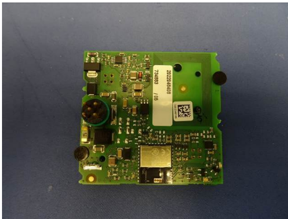
Top view of internal PCB
