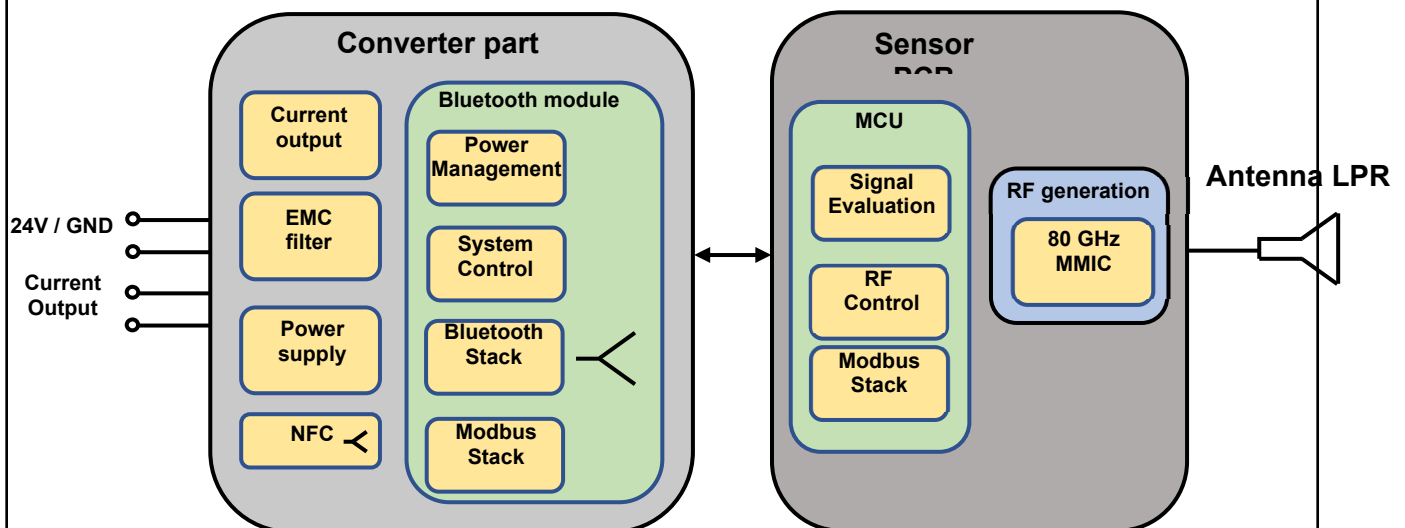
Figure 1: Block diagram DULCOLEVEL
