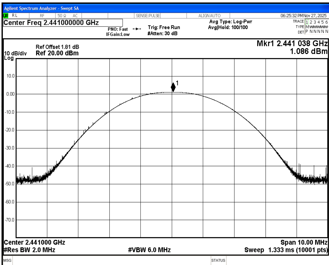
Power NVNT 1-DH5 2441MHz Ant1
