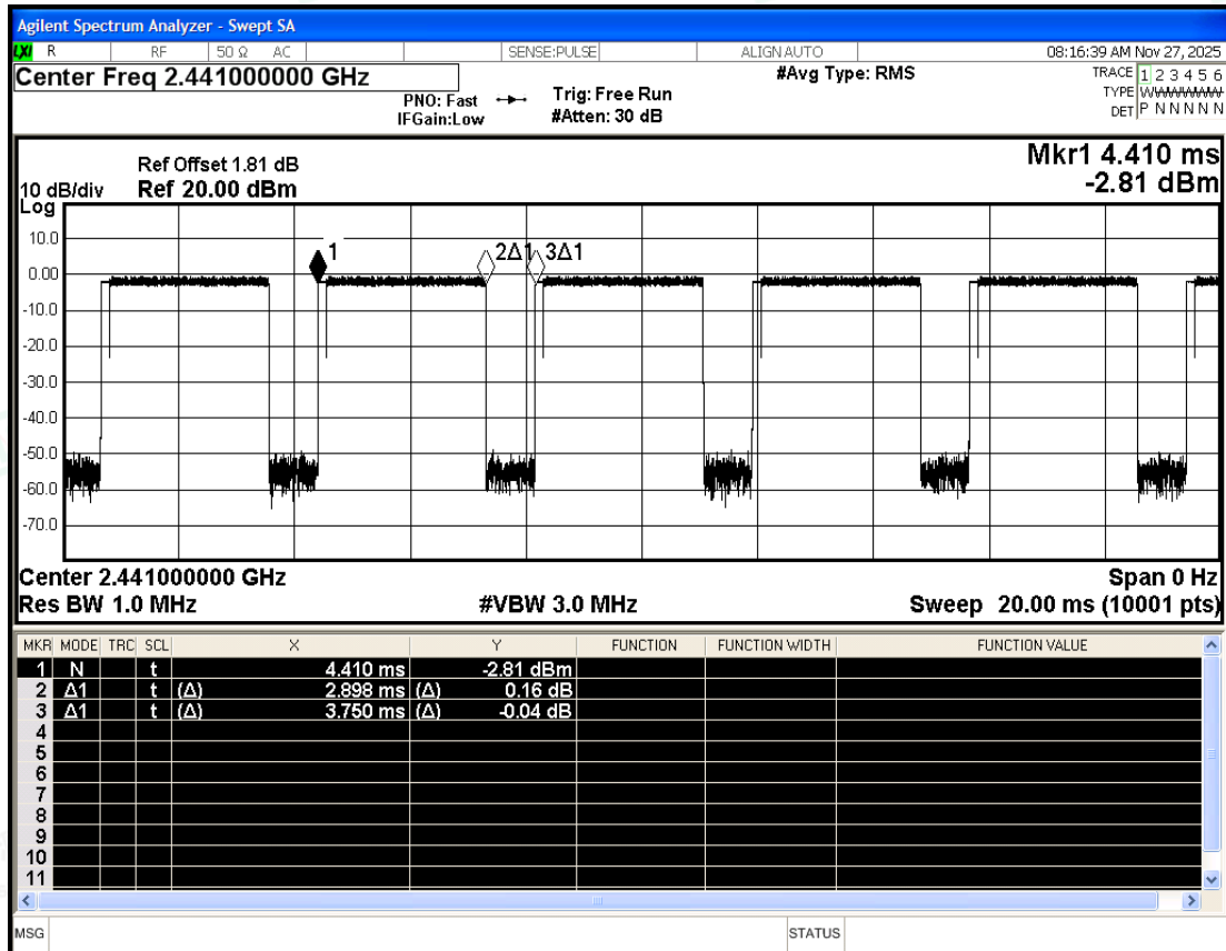
Duty Cycle NVNT 2-DH5 2441MHz Ant1
