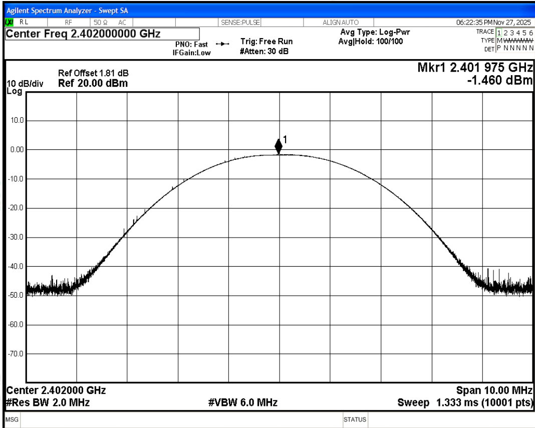
Power NVNT 1-DH5 2402MHz Ant1
