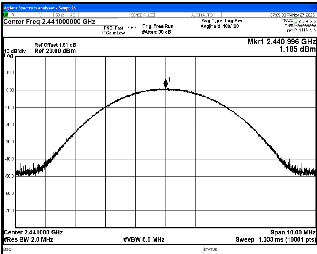
Power NVNT 3-DH5 2441MHz Ant1
