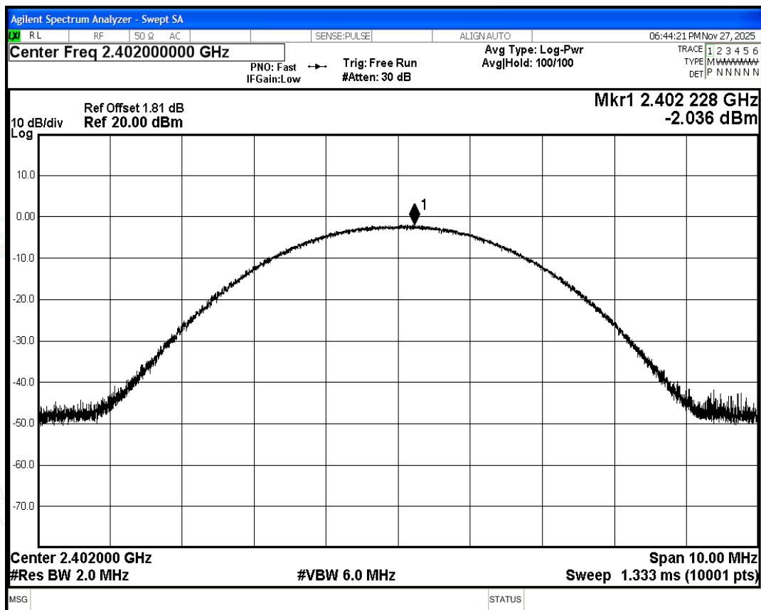
Power NVNT 2-DH5 2402MHz Ant1
