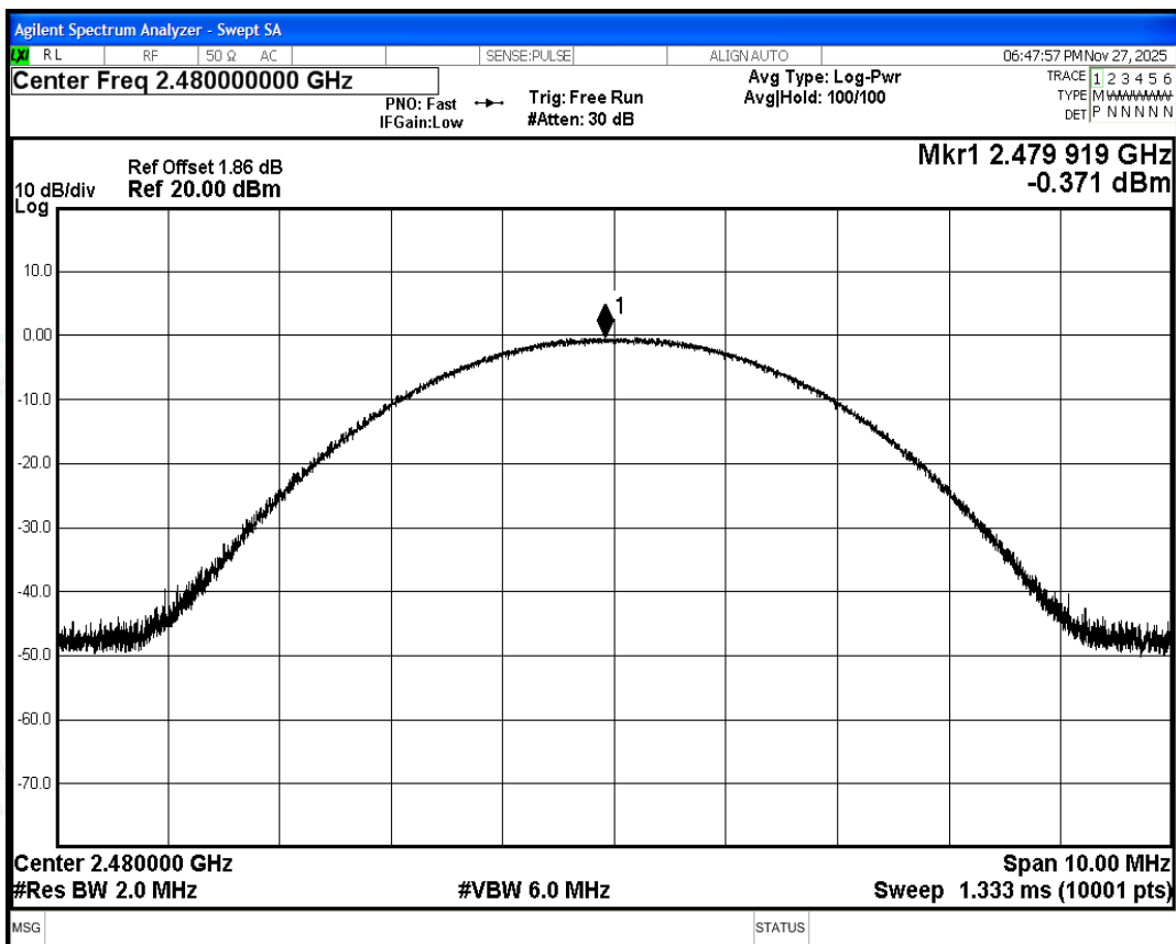
Power NVNT 2-DH5 2480MHz Ant1
