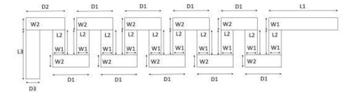
Antenna Dimensions
