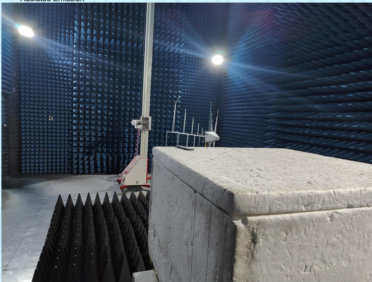
Radiated Emission
