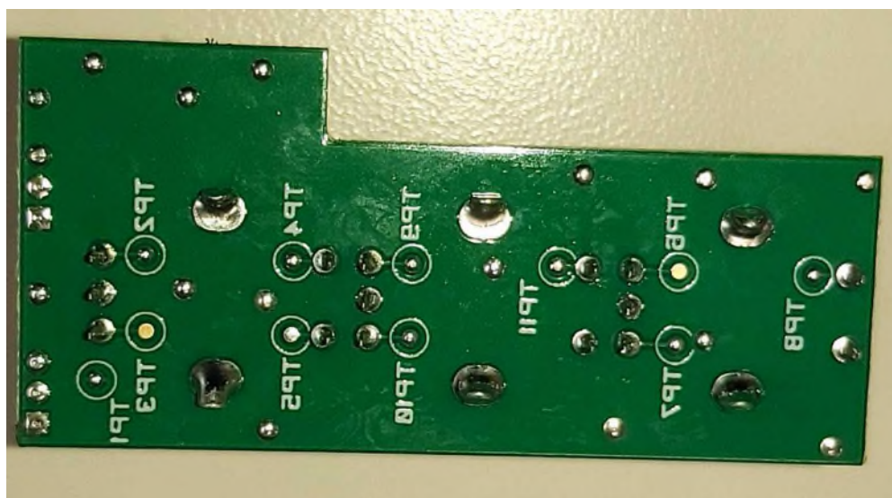
Figure 4 – Knob Board -Bottom
