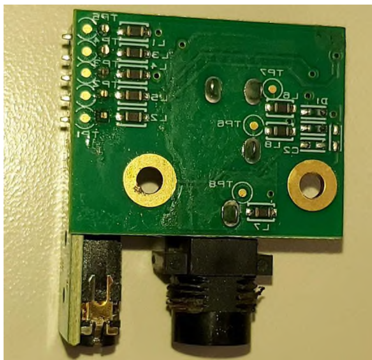
Figure 4 – Audio Input Board 1 -Bottom
