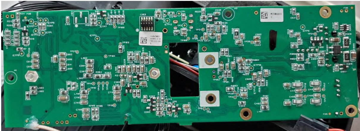
Figure 4 – Main PCB with Transmitter -Bottom
