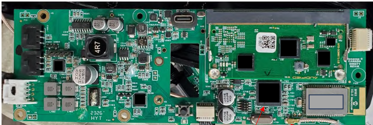
Figure 2 – Main PCB with Transmitter -Top
