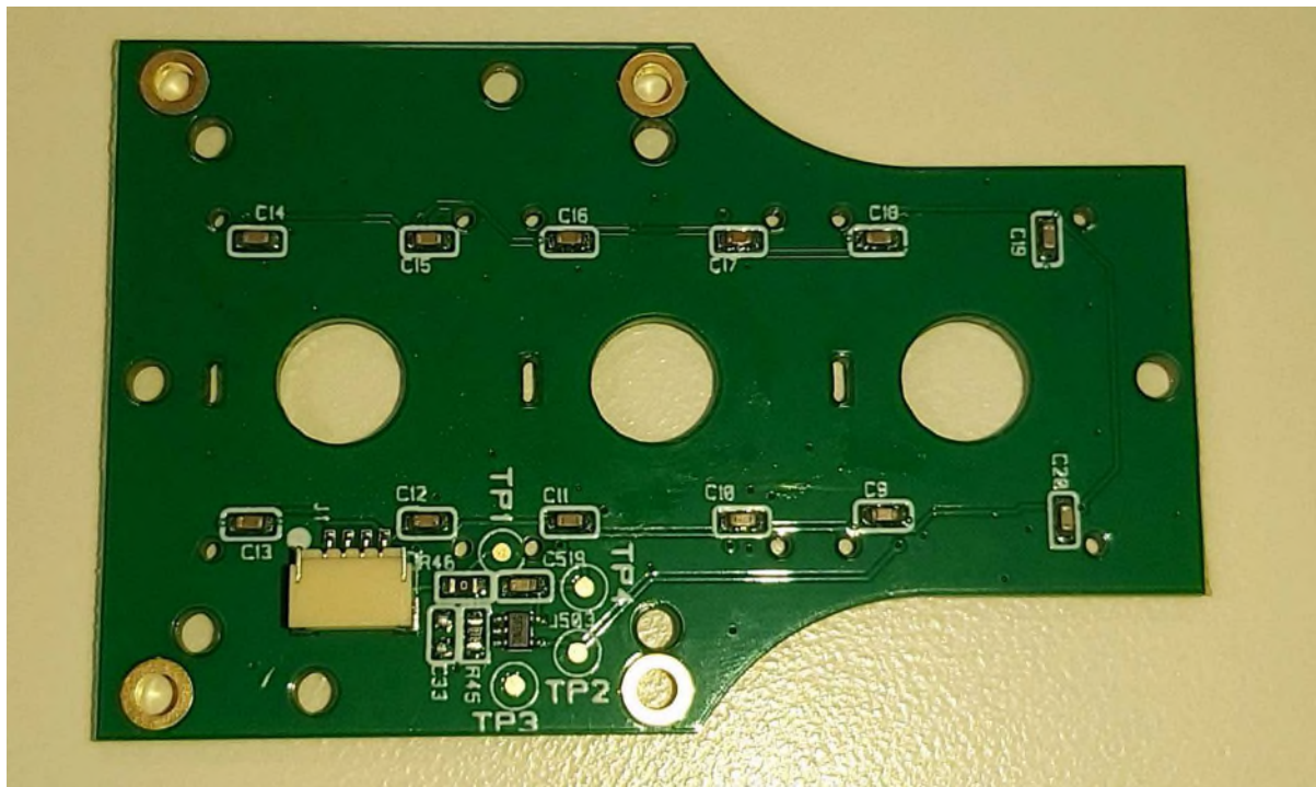
Figure 4 – LED Board -Top
