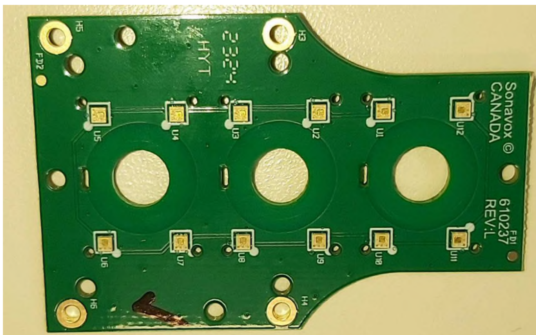
Figure 4 – LED Board -Bottom
