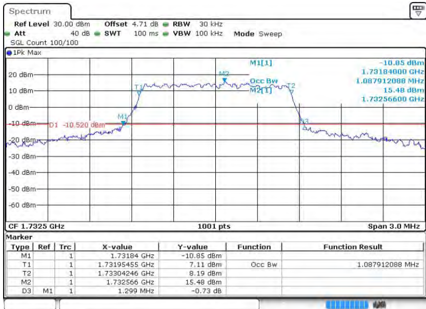
Band4-1.4MHz-QPSK-20175-6RB#0
