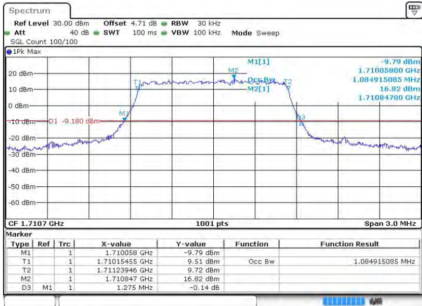
Band4-1.4MHz-QPSK-19957-6RB#0
