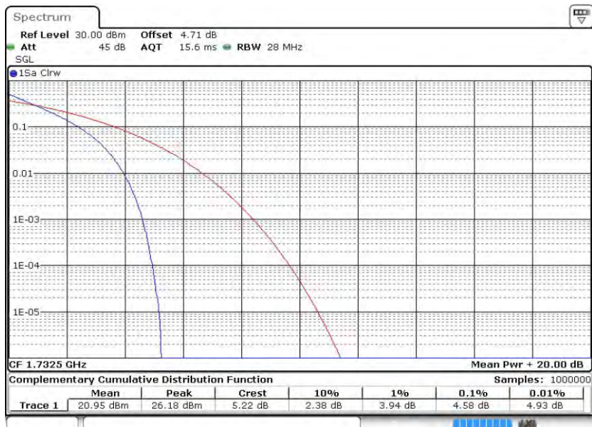
Band4-20MHz-QPSK-20175-100RB#0
