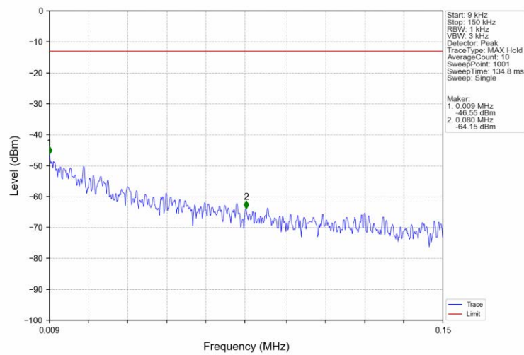
Band4_5MHz_QPSK_LCH_1712.5MHz_RB_1_0_NTNV
