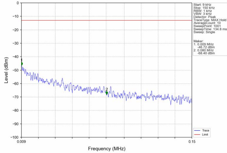
Band4_5MHz_16QAM_MCH_1732.5MHz_RB_1_0_NTNV
