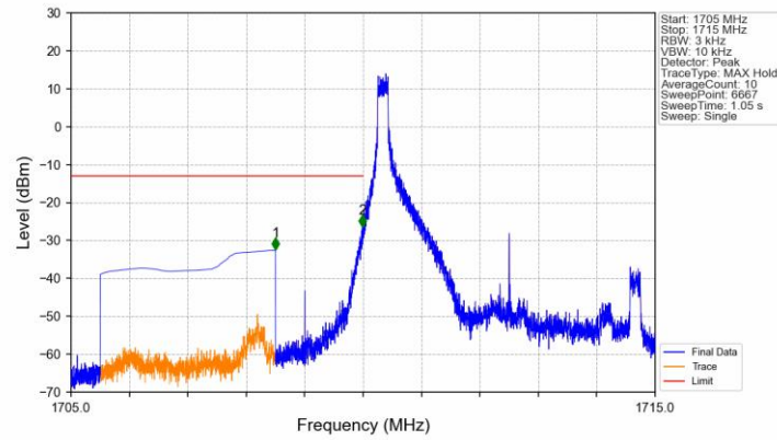
Band4_5MHz_QPSK_LCH_1712.5MHz_RB_1_0_NTNV
