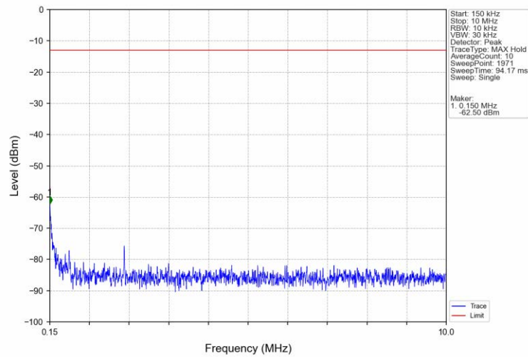
Band4_10MHz_16QAM_MCH_1732.5MHz_RB_1_0_NTNV
