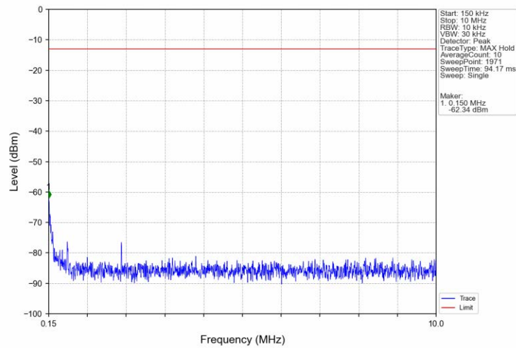
Band4_3MHz_16QAM_MCH_1732.5MHz_RB_1_0_NTNV
