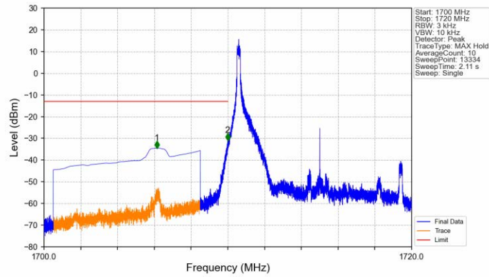
Band4_10MHz_QPSK_LCH_1715MHz_RB_1_0_NTNV
