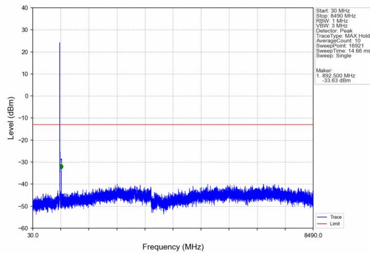
Band5_5MHz_16QAM_HCH_846.5MHz_RB_1_0_NTNV
