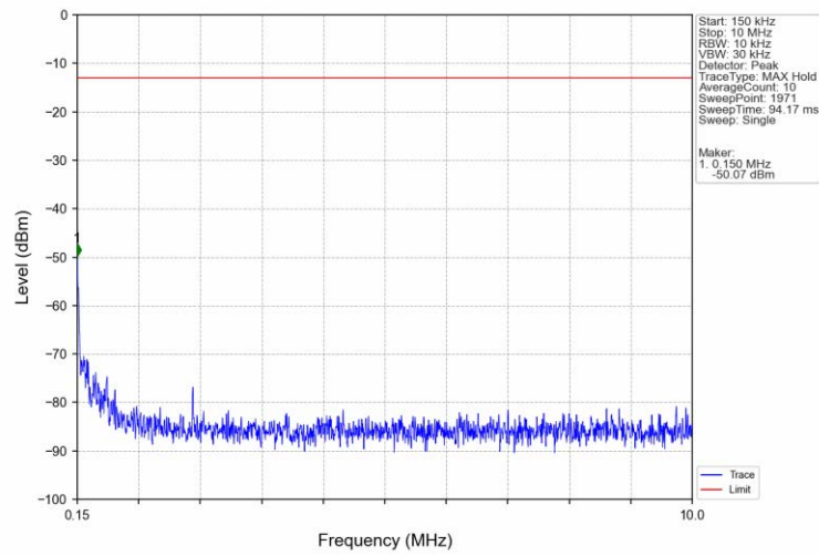
Band5_10MHz_16QAM_HCH_844MHz_RB_1_0_NTNV
