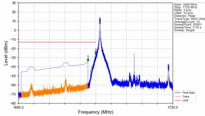
Band66_15MHz_QPSK_LCH_1717.5MHz_RB_1_0_NTNV
