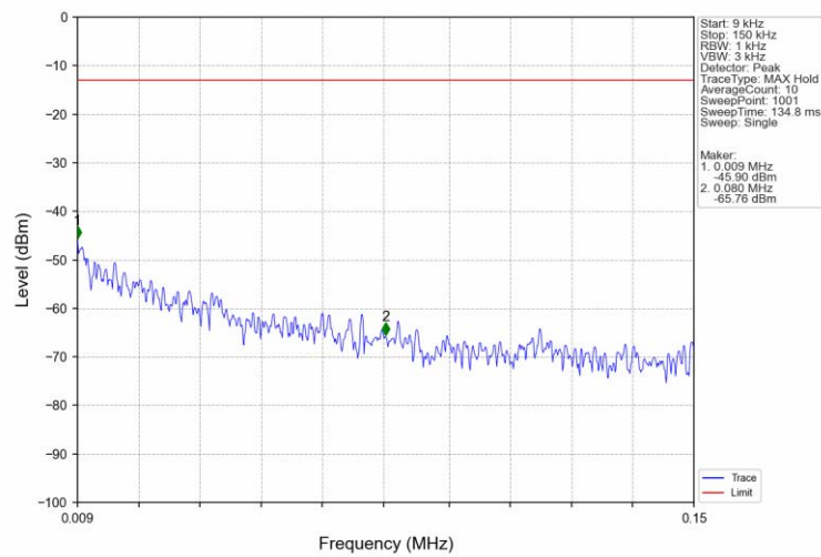
Band66_3MHz_QPSK_LCH_1711.5MHz_RB_1_0_NTNV
