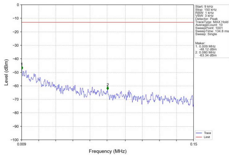
Band66_5MHz_QPSK_LCH_1712.5MHz_RB_1_0_NTNV
