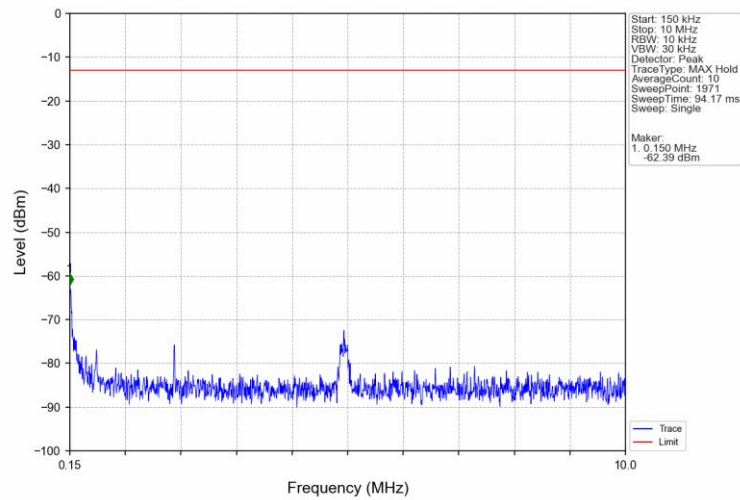
Band66_15MHz_16QAM_LCH_1717.5MHz_RB_1_0_NTNV
