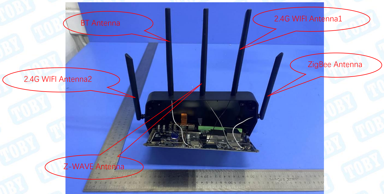
Photo 11 Appearance of PCB
