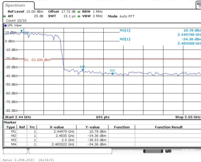
11AX40MIMO_Ant2_High_2452_Peak
