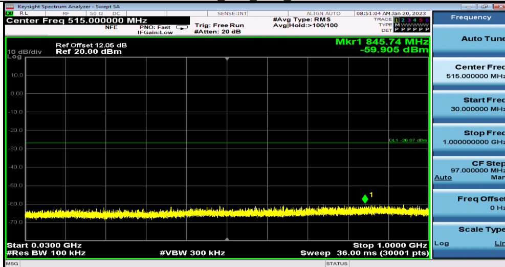
11N20SISO Ant1 2412 30-1000
