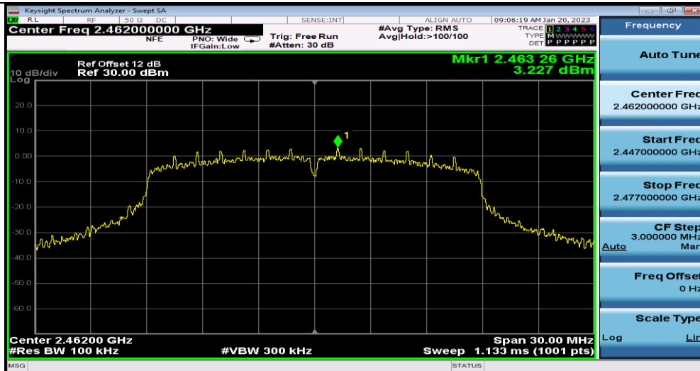
11N20SISO Ant1 2462 0~Reference
