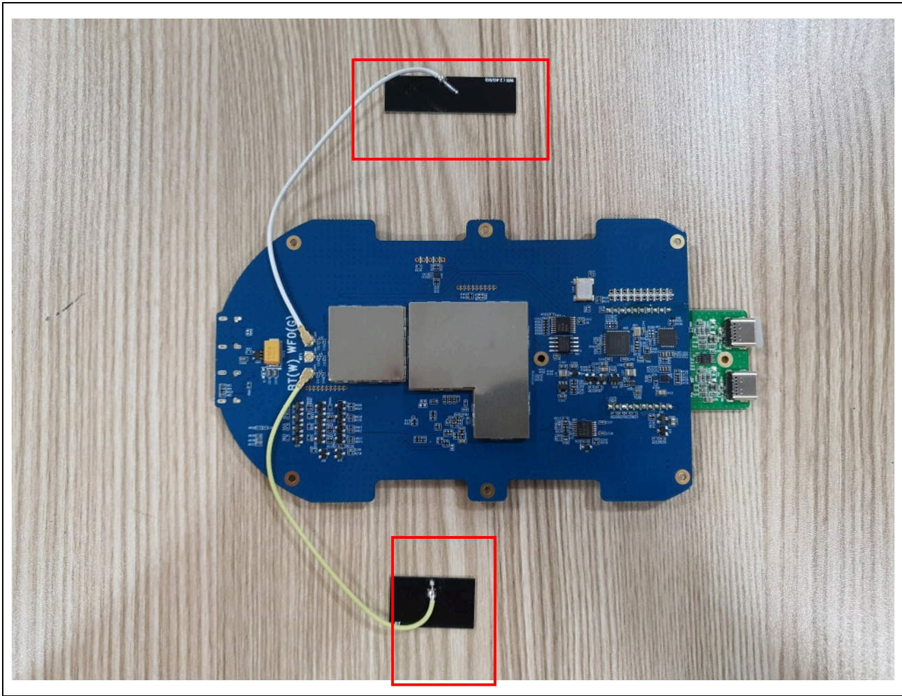
Antenna(2.4GHz, 5 GHz ANT)
