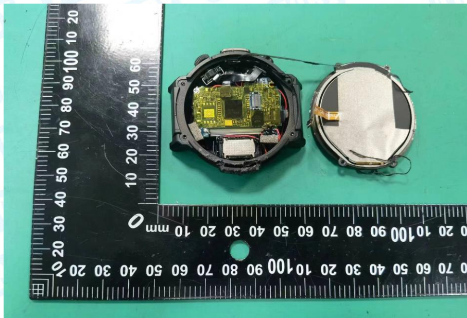
Photo 9 Internal of EUT
