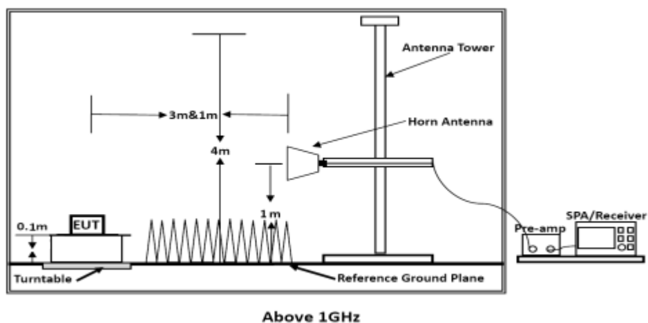
Figure 3. Above 1GHz
