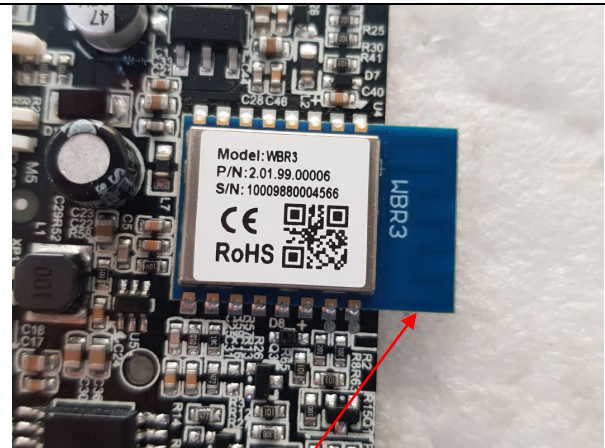
Pattern Antenna
