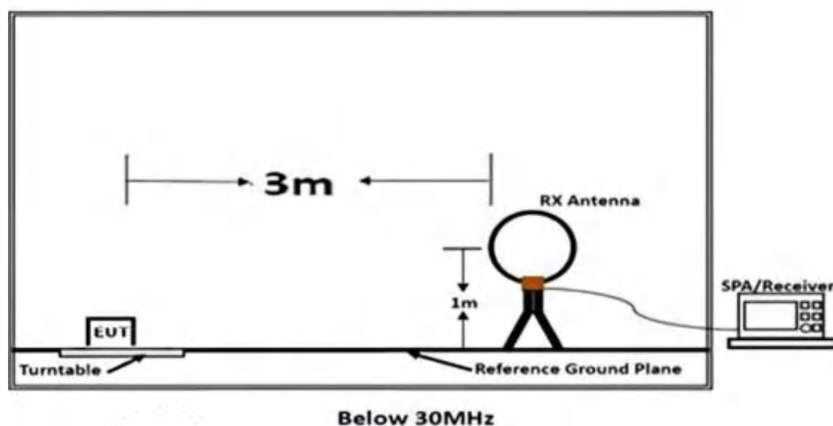
Below 30MHz Test Setup
