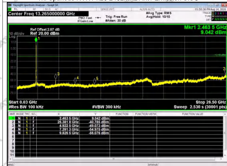
Tx. Spurious NVNT n20 2462MHz Ant1 Emission SISO
