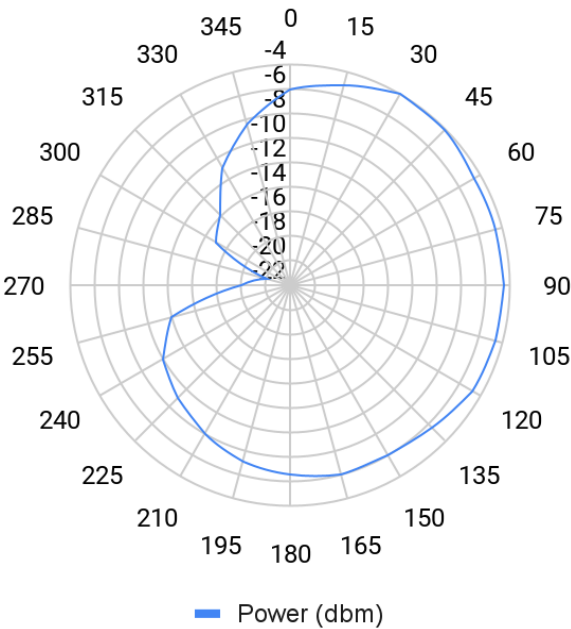
Fig 5.1.3 Free Space EIRP (2450 MHz) - XY Cut
