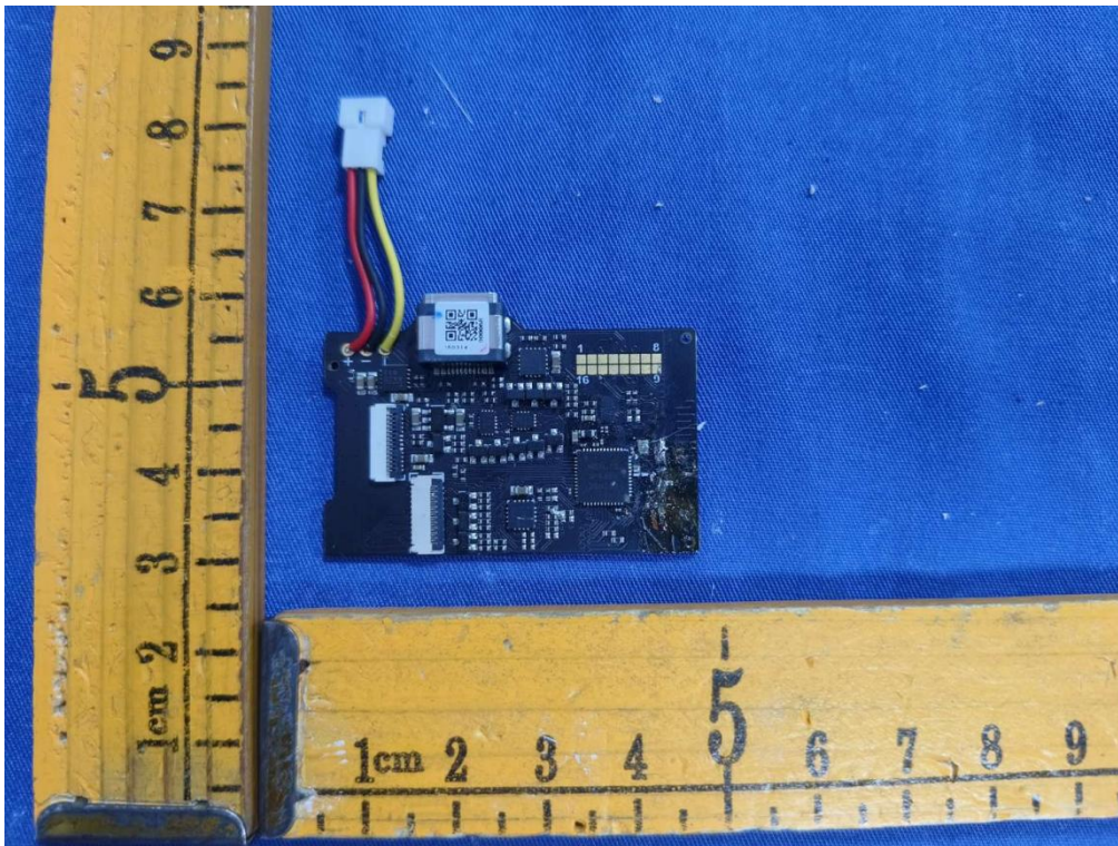
Internal view of unit (Model:RKN-T1M-25-002)
