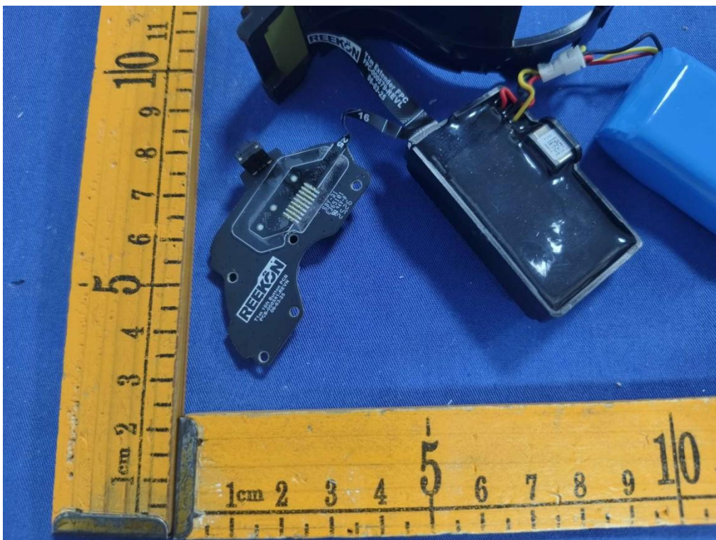
Internal view of unit (Model:RKN-T1M-16-002)
