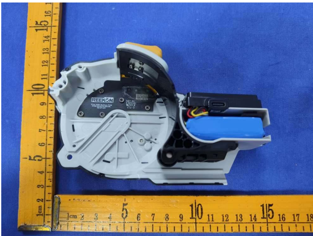
Internal view of unit (Model:RKN-T1M-25-001)
