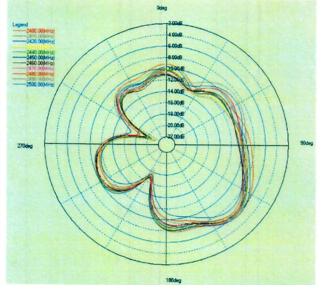
Horizontal Radiation Pattern
