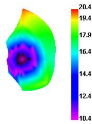
Wifi 7 TRP
