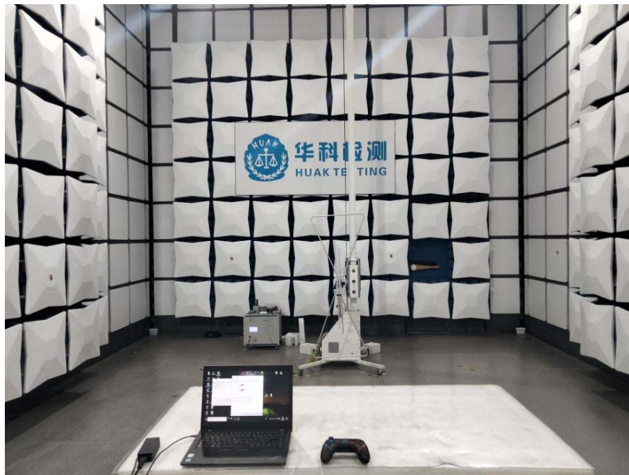
Model: S10-S Radiated Emissions
