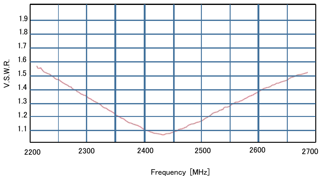
Fig.1 驻波比 VSWR
