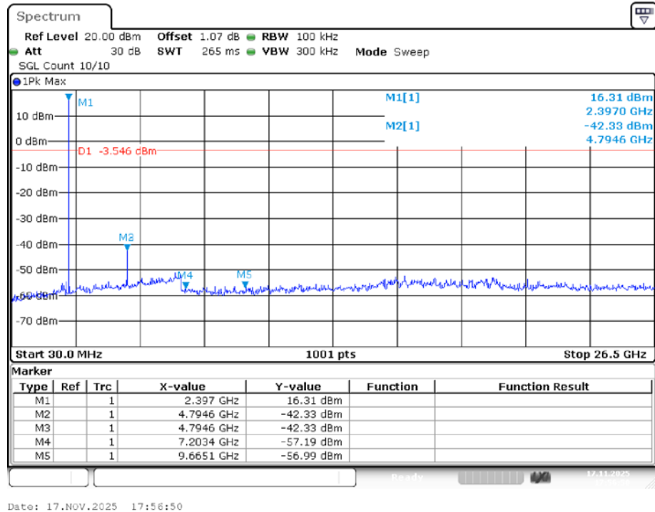
Tx. Spurious NVNT LORA 2405MHz Ant1 Emission
