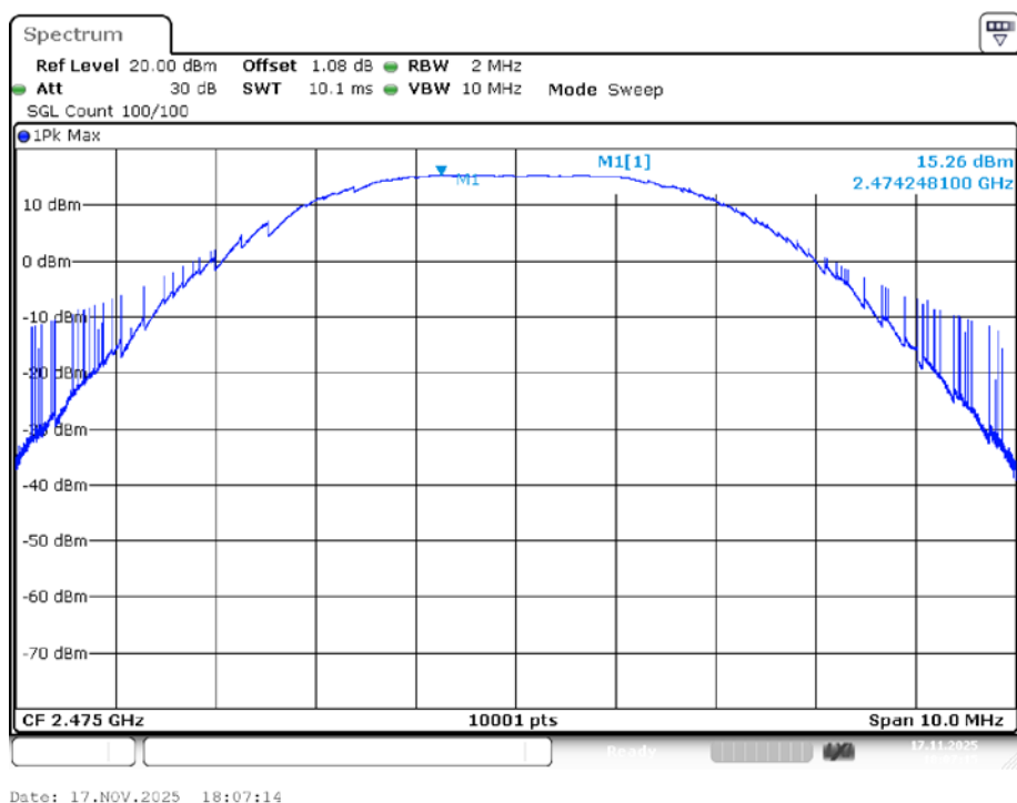
Power NVNT LORA 2475MHz Ant1
