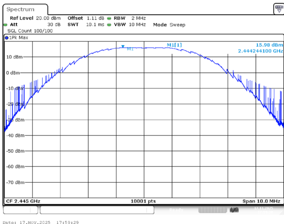
Power NVNT LORA 2445MHz Ant1
