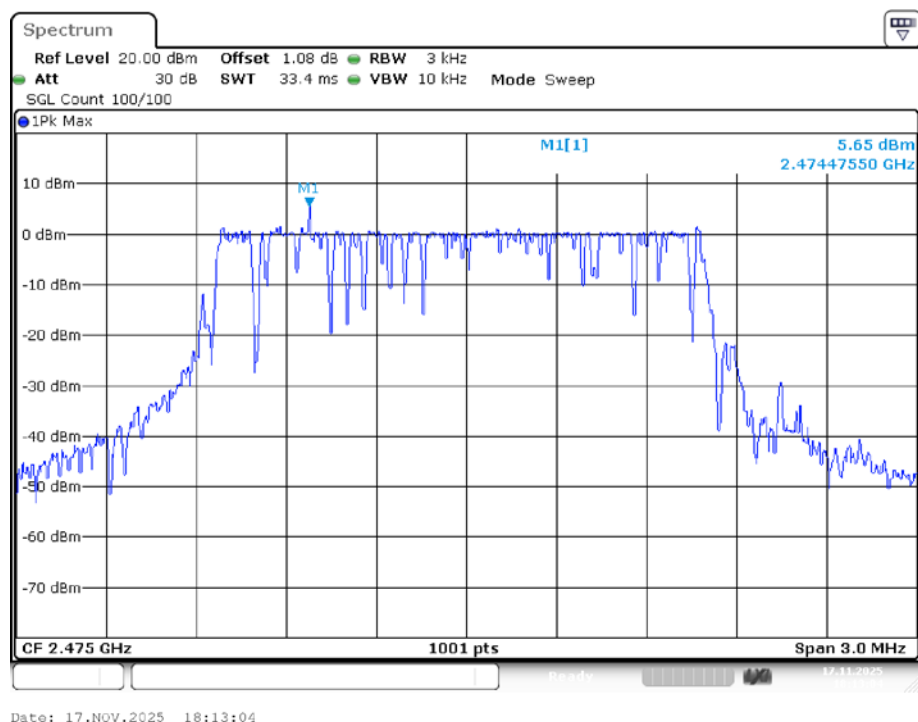
PSD NVNT LORA 2475MHz Ant1
