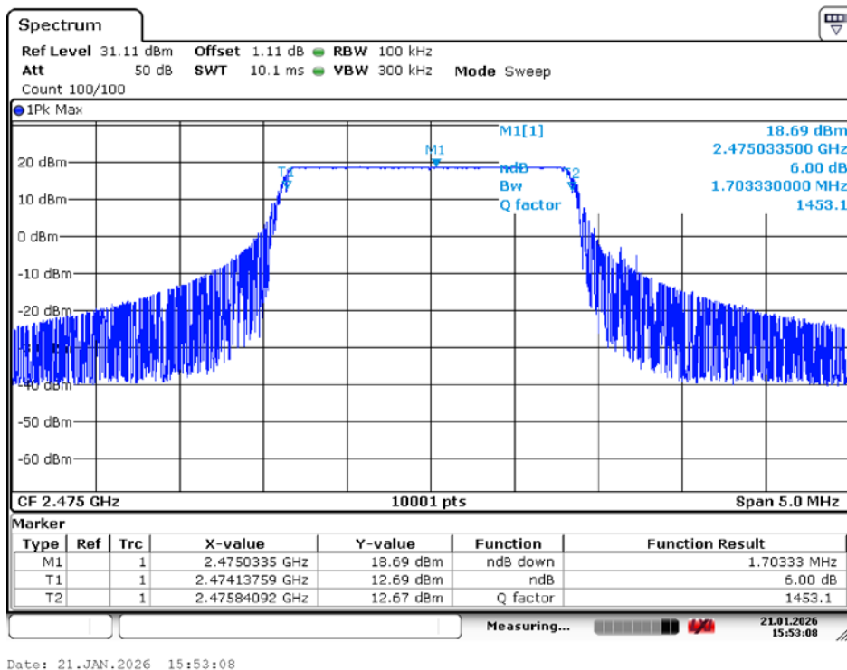
-6dB Bandwidth NVNT LORA 2475MHz Ant1
