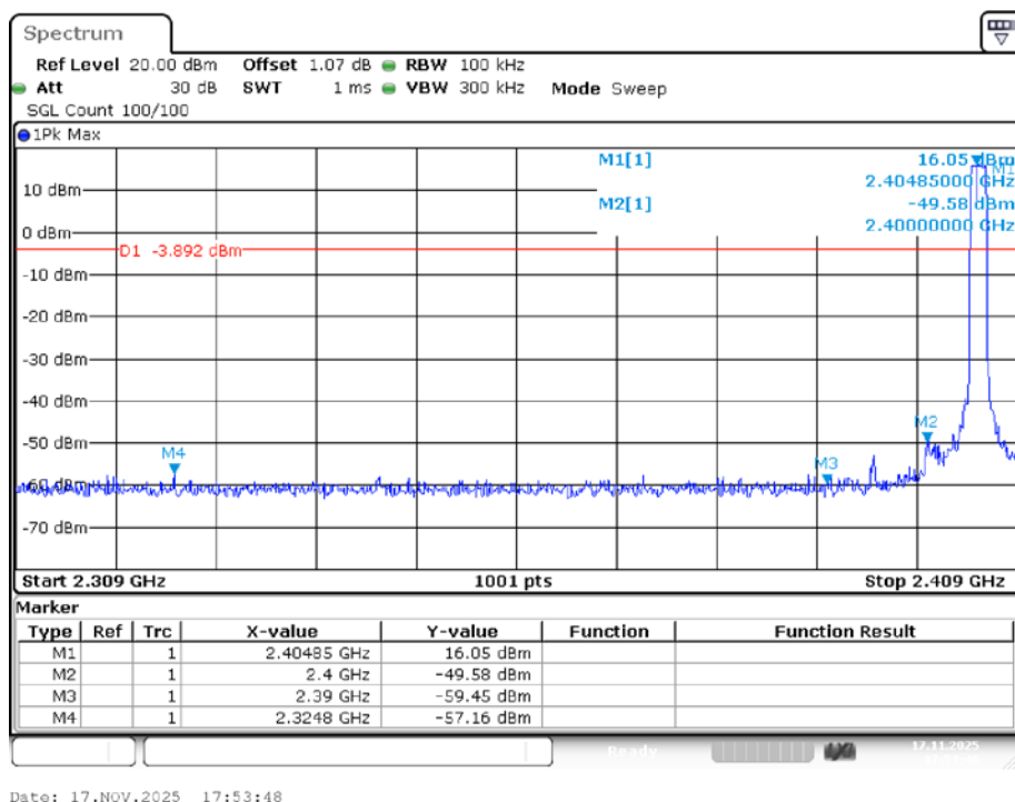
Band Edge NVNT LORA 2405MHz Ant1 Emission
