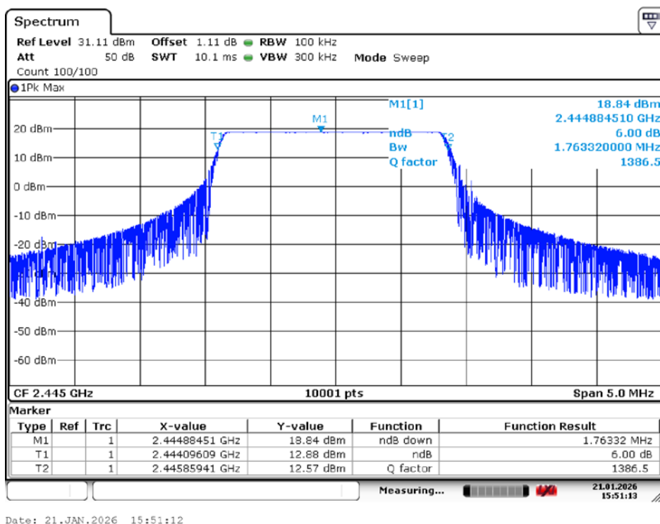
-6dB Bandwidth NVNT LORA 2445MHz Ant1
