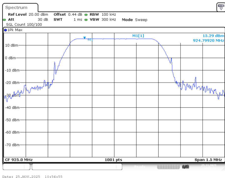
Tx. Spurious NVNT LORA 925MHz Ant1 Ref
