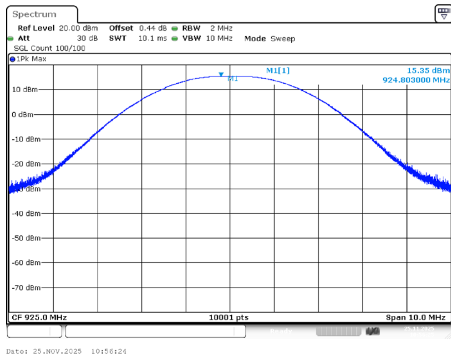
Power NVNT LORA 925MHz Ant1
