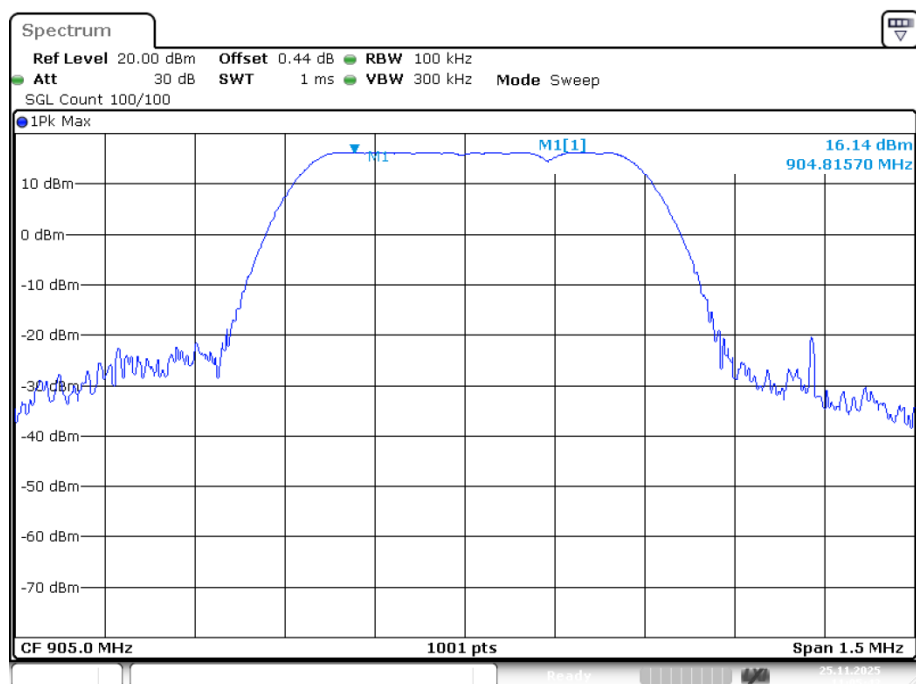
Tx. Spurious NVNT LORA 905MHz Ant1 Ref
