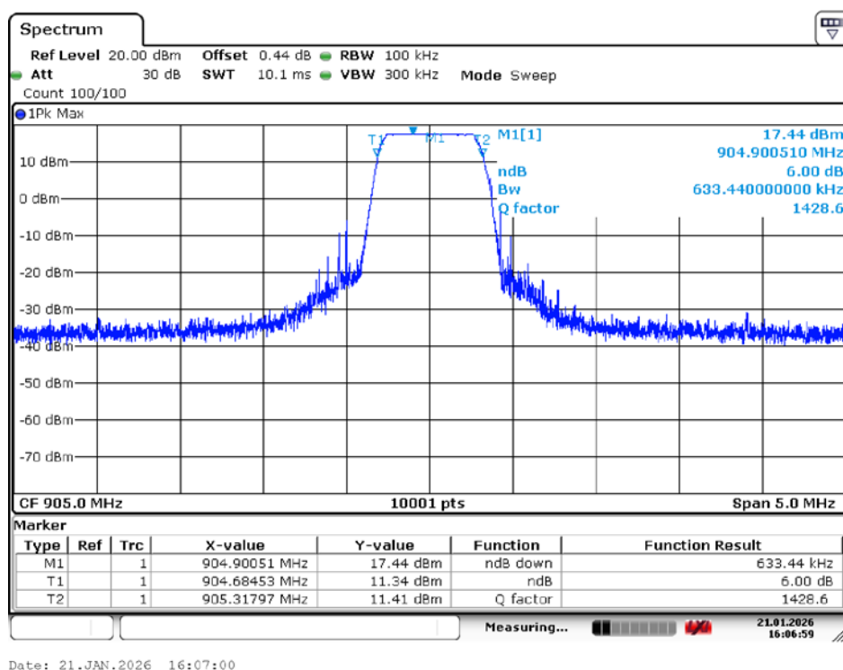
-6dB Bandwidth NVNT LORA 905MHz Ant1
