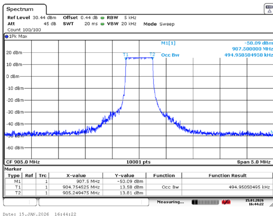
OBW NVNT LORA 905MHz Ant1
