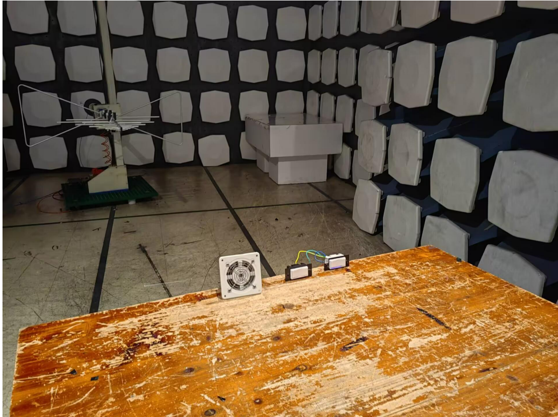
30 MHz to 1 GHz Radiated Spurious Emissions
