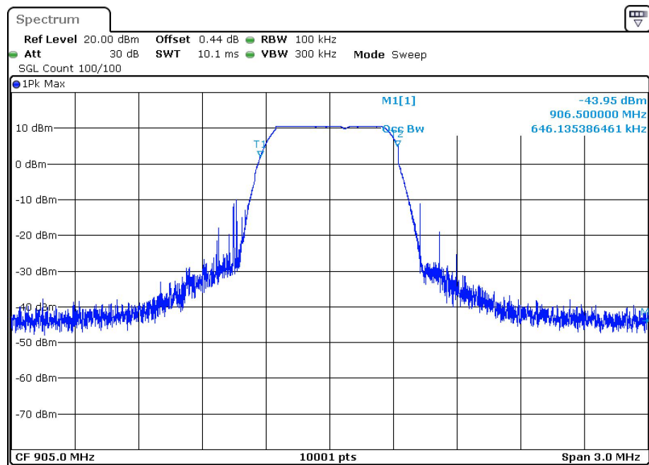
OBW NVNT LORA 905MHz Ant1
