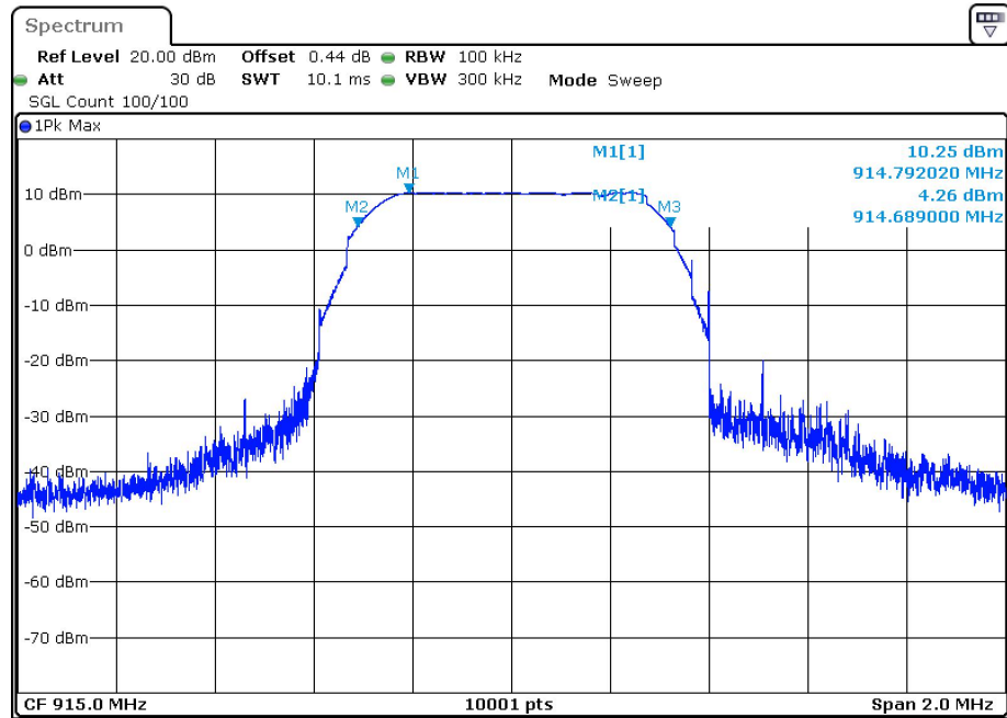
-6dB Bandwidth NVNT LORA 915MHz Ant1
