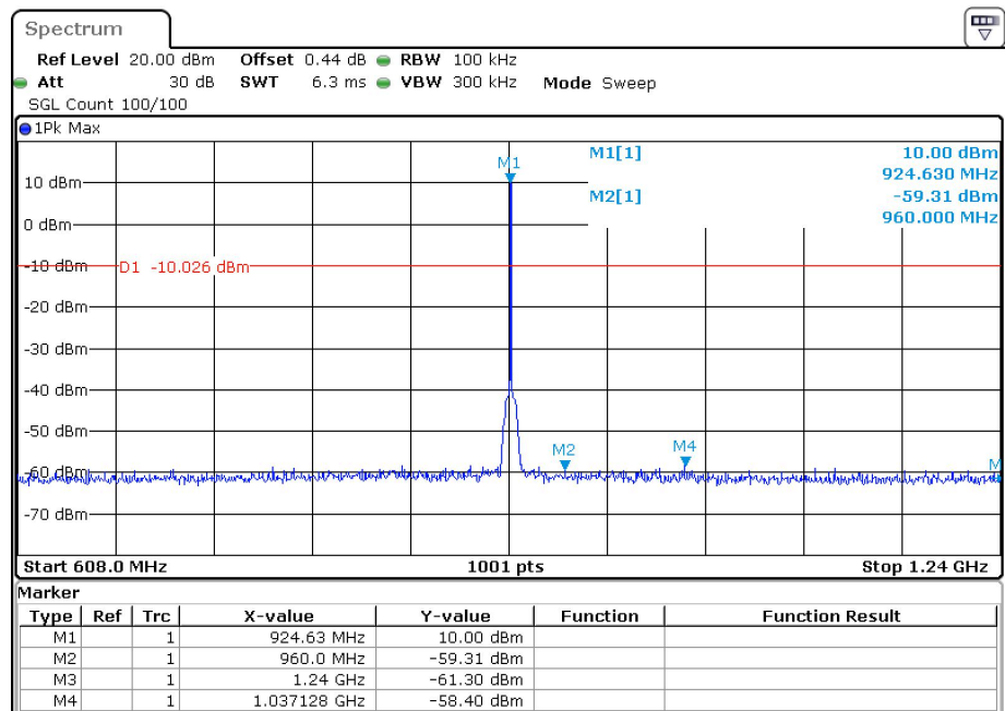
Band Edge NVNT LORA 925MHz Ant1 Emission
