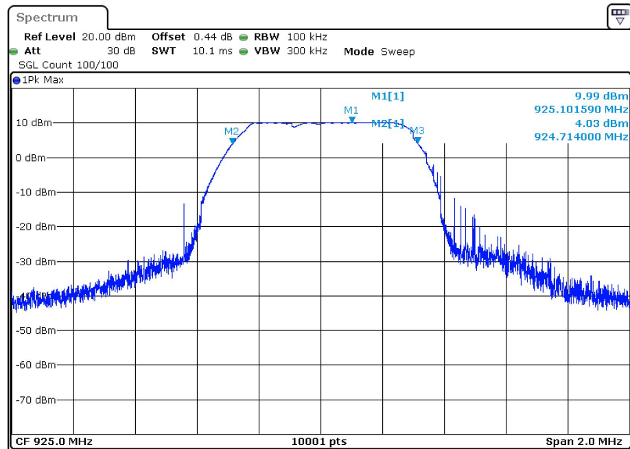
-6dB Bandwidth NVNT LORA 925MHz Ant1
