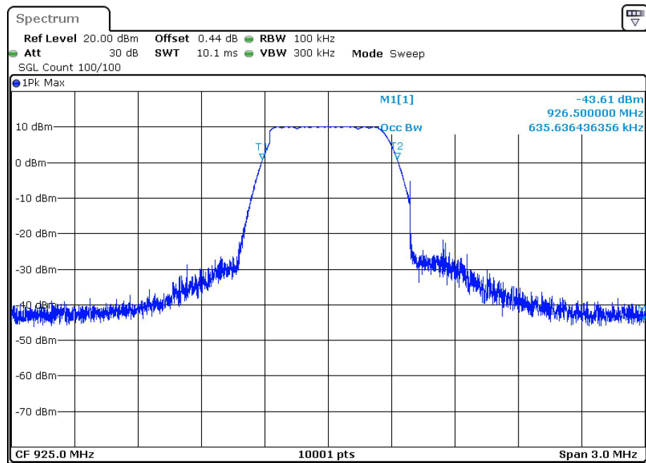
OBW NVNT LORA 925MHz Ant1
