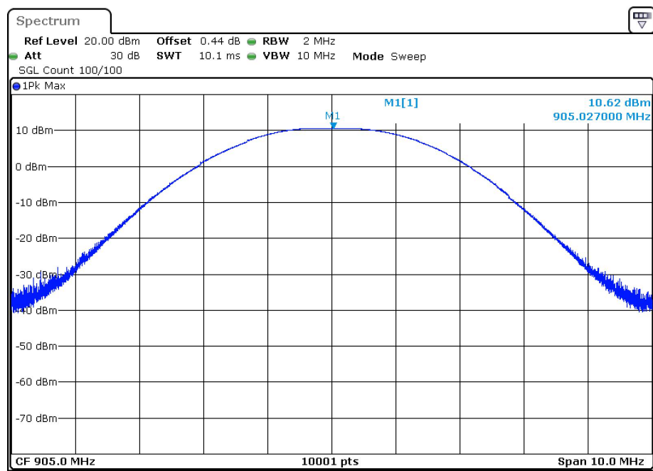
Power NVNT LORA 905MHz Ant1
