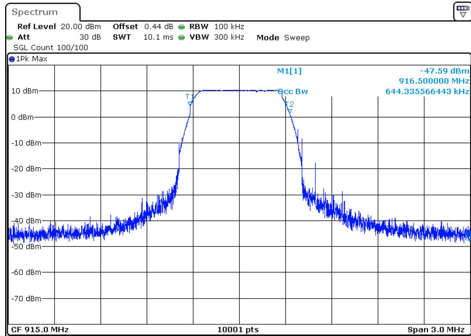
OBW NVNT LORA 915MHz Ant1
