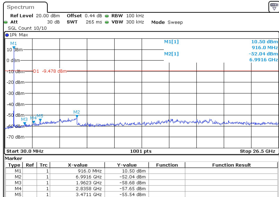
Tx. Spurious NVNT LORA 905MHz Ant1 Emission
