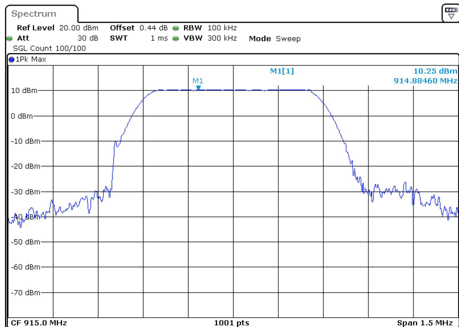
Tx. Spurious NVNT LORA 915MHz Ant1 Ref
