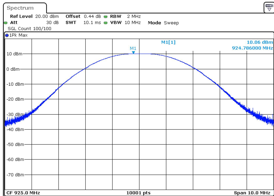
Power NVNT LORA 925MHz Ant1
