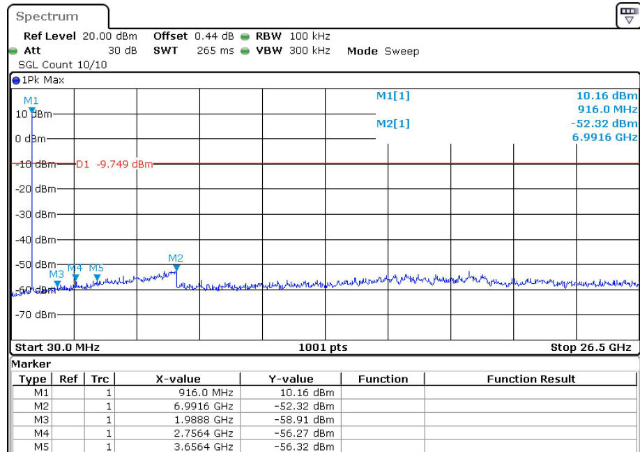
Tx. Spurious NVNT LORA 915MHz Ant1 Emission
