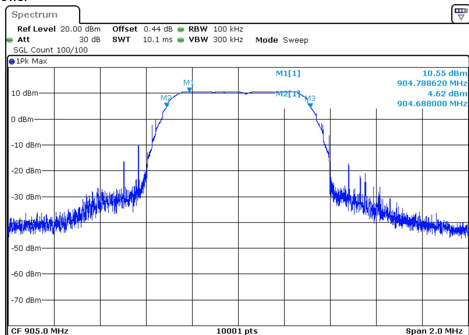
-6dB Bandwidth NVNT LORA 905MHz Ant1
