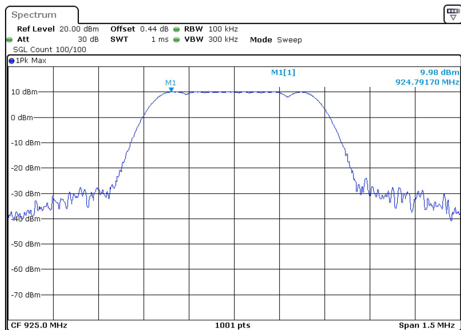
Tx. Spurious NVNT LORA 925MHz Ant1 Ref
