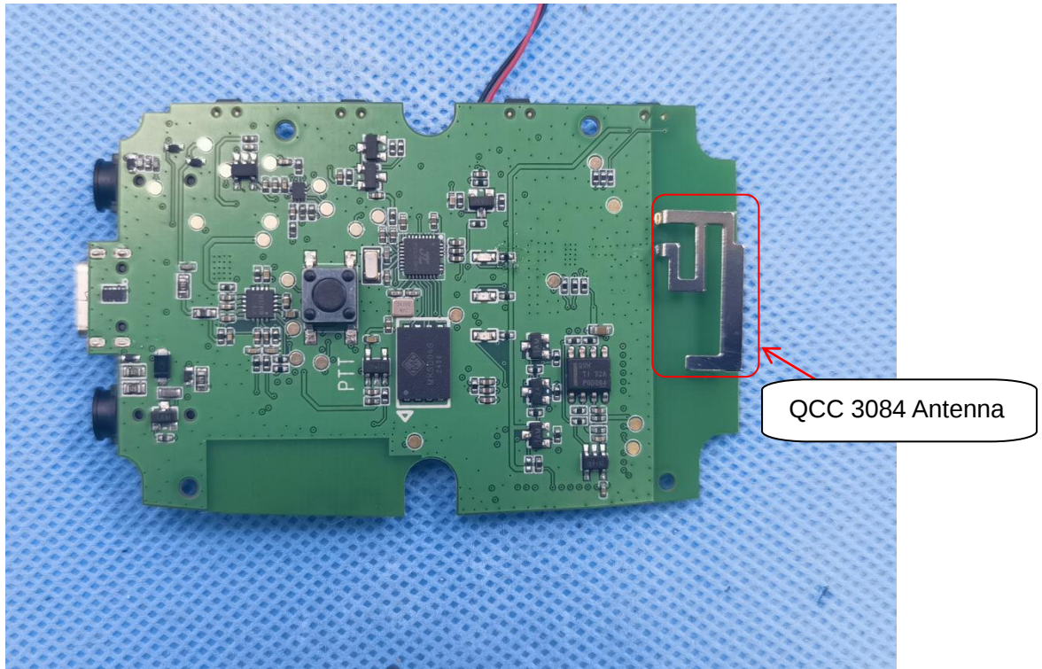
INTERNAL VIEW OF EUT (FIGURE 5)
