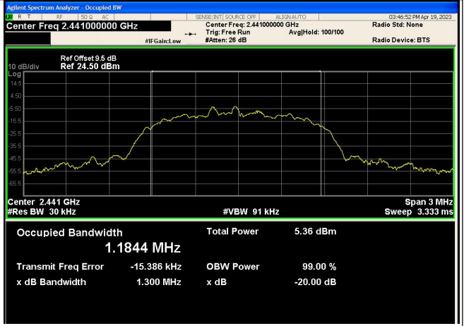
8DPSK_3-DH5_Channel 39
