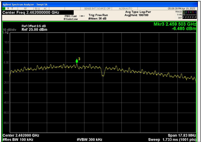
In-Band Reference Level IEEE 802.11n_Channel 11_20MHz_Antenna 0
