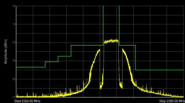
Band40(2350-2360) QAM16 BW=5MHz Channel=39225 RB Size=25 Position=#0
