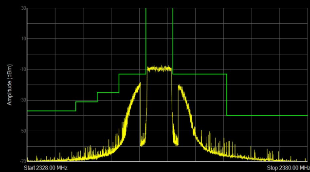
Band40(2350-2360) QAM16 BW=5MHz Channel=39175 RB Size=25 Position=#0
