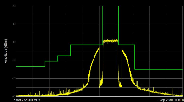
Band40(2350-2360) QPSK BW=5MHz Channel=39225 RB Size=25 Position=#0
