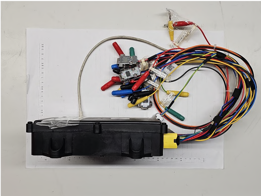
Photograph 2: EUT 1_Side view with cables attached
