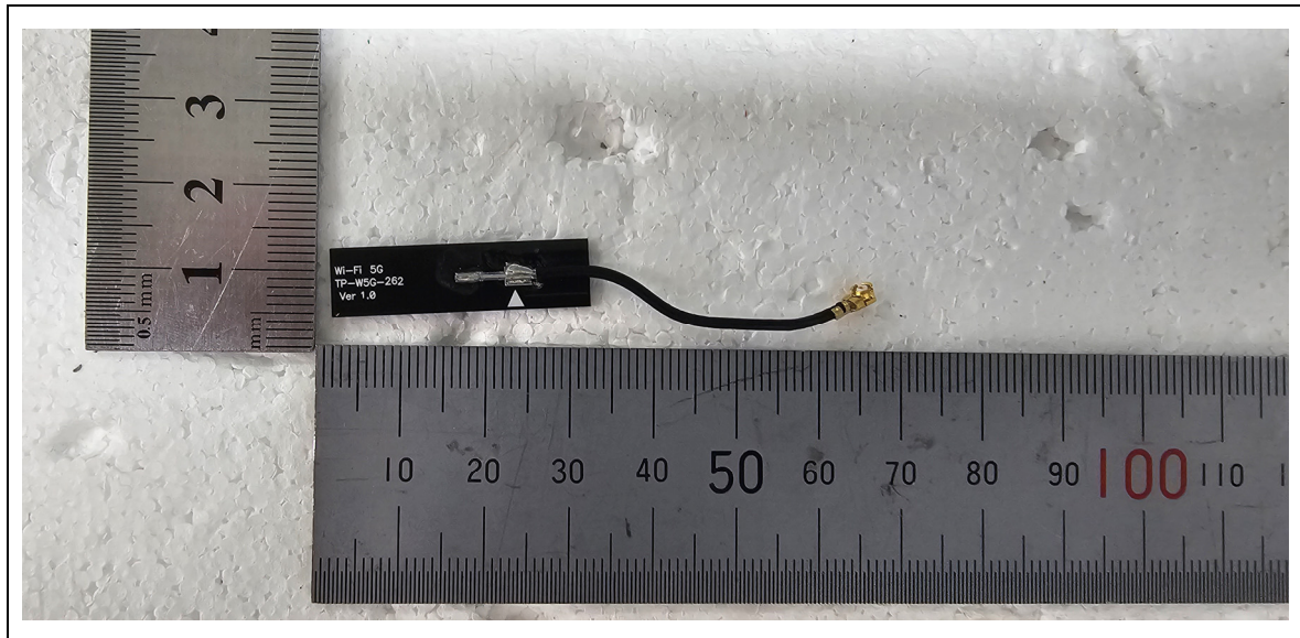
<WLAN Antenna 1>
